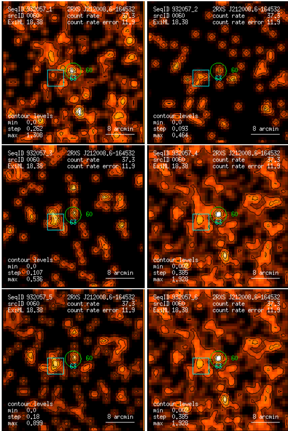
Figure 60: RASS 932057: detection 0060: band rate images, Gaussian filter: (1) PSPC channels 11 – 41, (2) 52 – 90, (3) 91 – 201, (4) 11 – 235, (5) 52 – 201, (6) 11 – 201. Broad band rates in counts/ks. Band rate contour levels in counts/ks/arcmin 2 .
