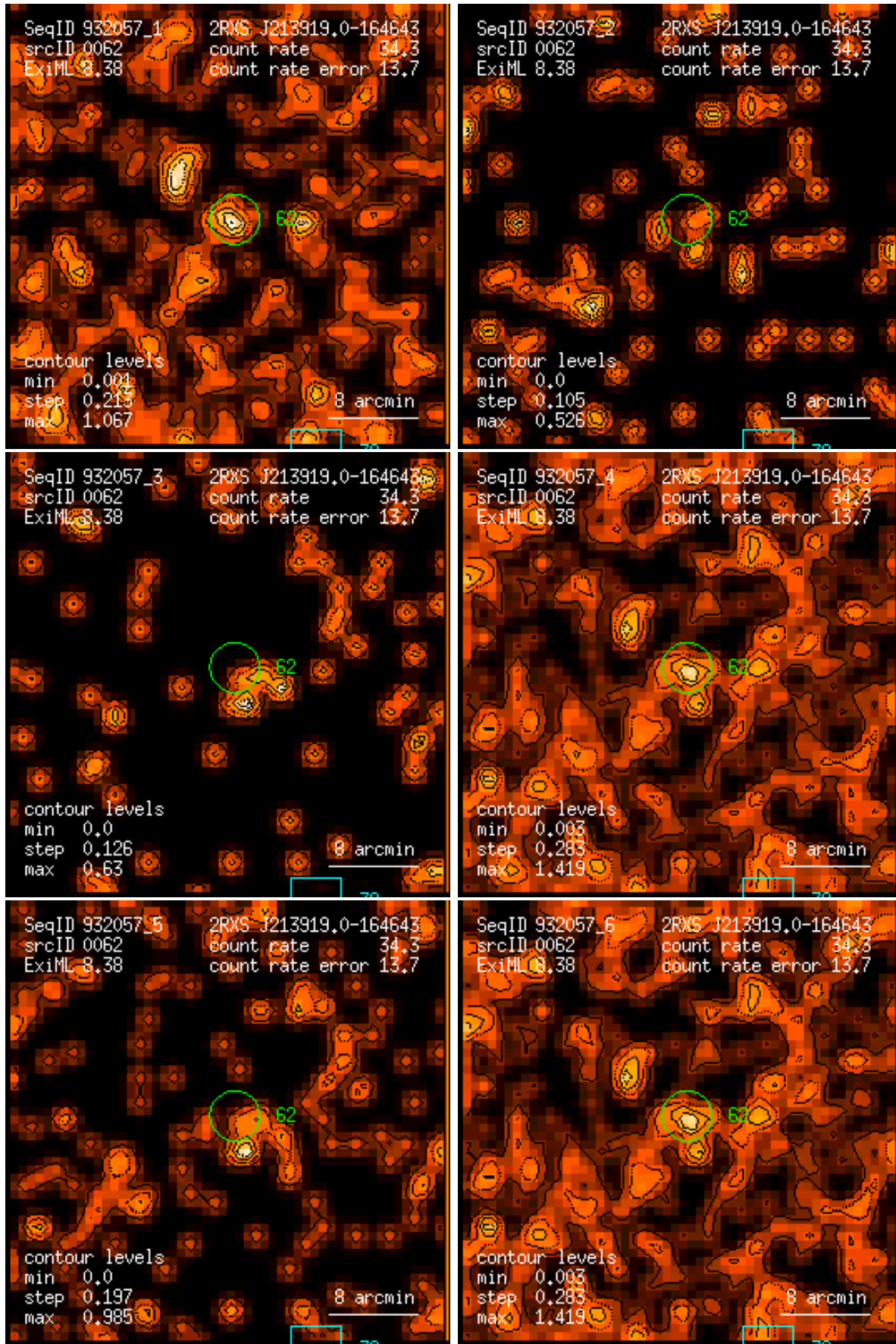
Figure 62: RASS 932057: detection 0062: band rate images, Gaussian filter: (1) PSPC channels 11 – 41, (2) 52 – 90, (3) 91 – 201, (4) 11 – 235, (5) 52 – 201, (6) 11 – 201. Broad band rates in counts/ks. Band rate contour levels in counts/ks/arcmin 2 .
