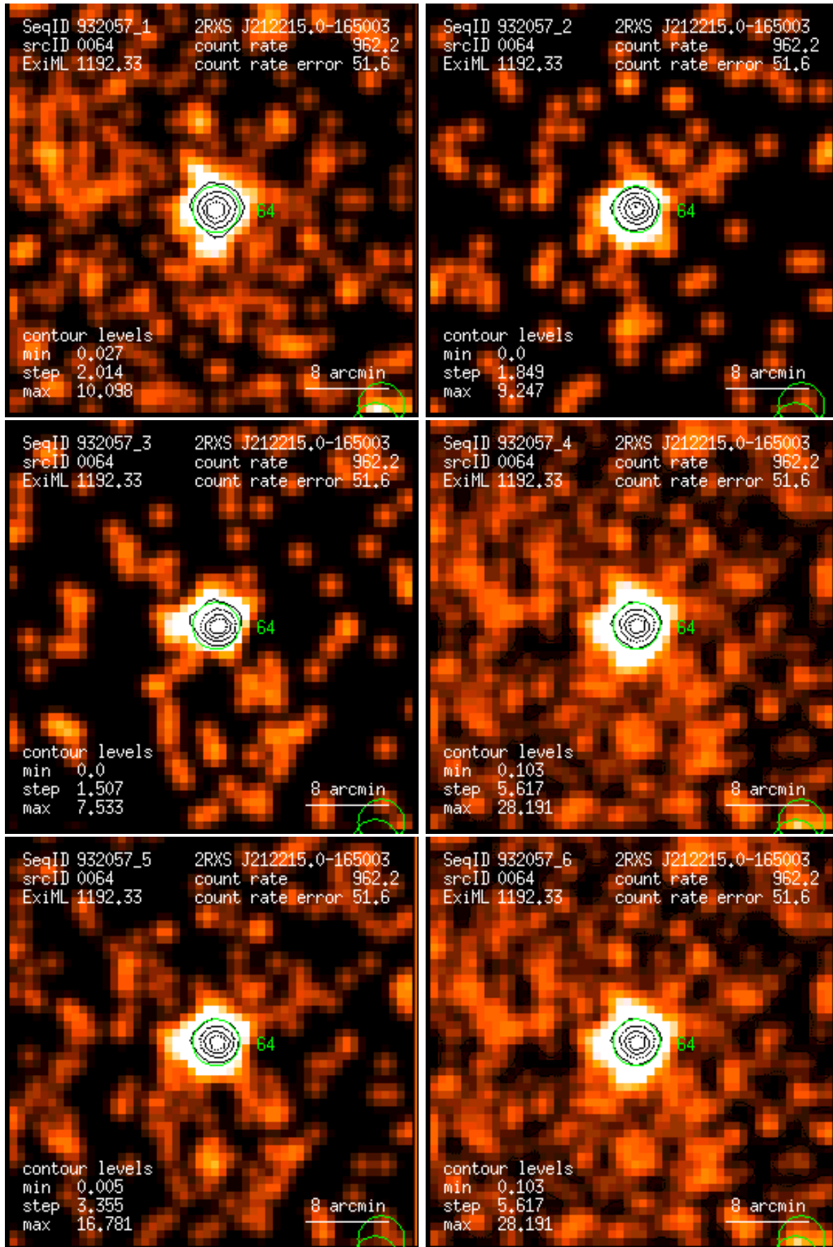
Figure 64: RASS 932057: detection 0064: band rate images, Gaussian filter: (1) PSPC channels 11 – 41, (2) 52 – 90, (3) 91 – 201, (4) 11 – 235, (5) 52 – 201, (6) 11 – 201. Broad band rates in counts/ks. Band rate contour levels in counts/ks/arcmin 2 .
