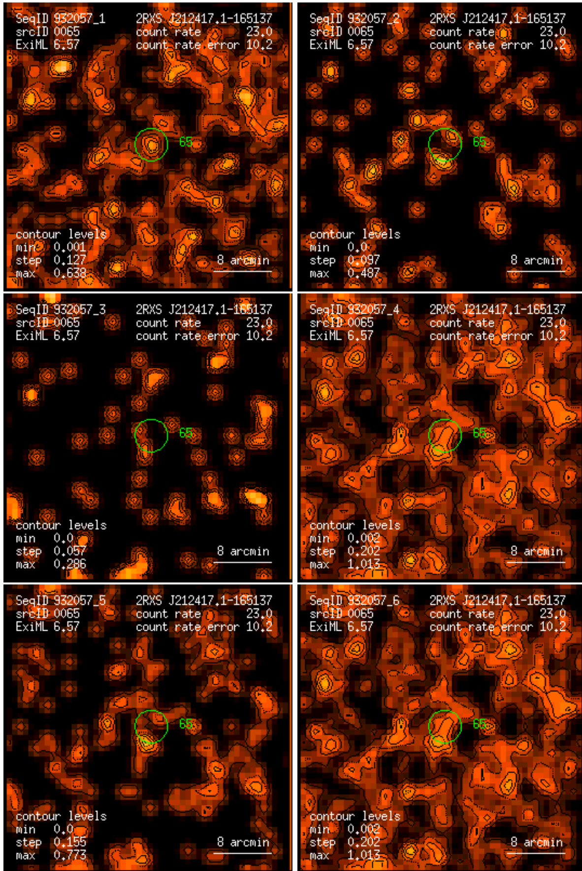
Figure 65: RASS 932057: detection 0065: band rate images, Gaussian filter: (1) PSPC channels 11 – 41, (2) 52 – 90, (3) 91 – 201, (4) 11 – 235, (5) 52 – 201, (6) 11 – 201. Broad band rates in counts/ks. Band rate contour levels in counts/ks/arcmin 2 .
