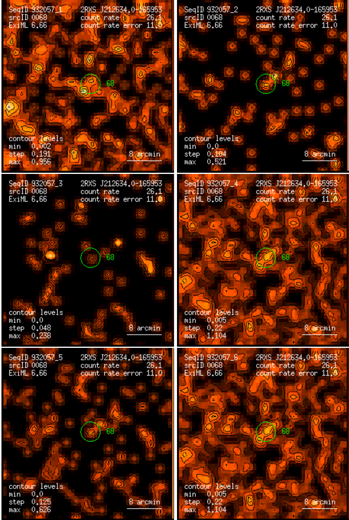
Figure 68: RASS 932057: detection 0068: band rate images, Gaussian filter: (1) PSPC channels 11 – 41, (2) 52 – 90, (3) 91 – 201, (4) 11 – 235, (5) 52 – 201, (6) 11 – 201. Broad band rates in counts/ks. Band rate contour levels in counts/ks/arcmin 2 .
