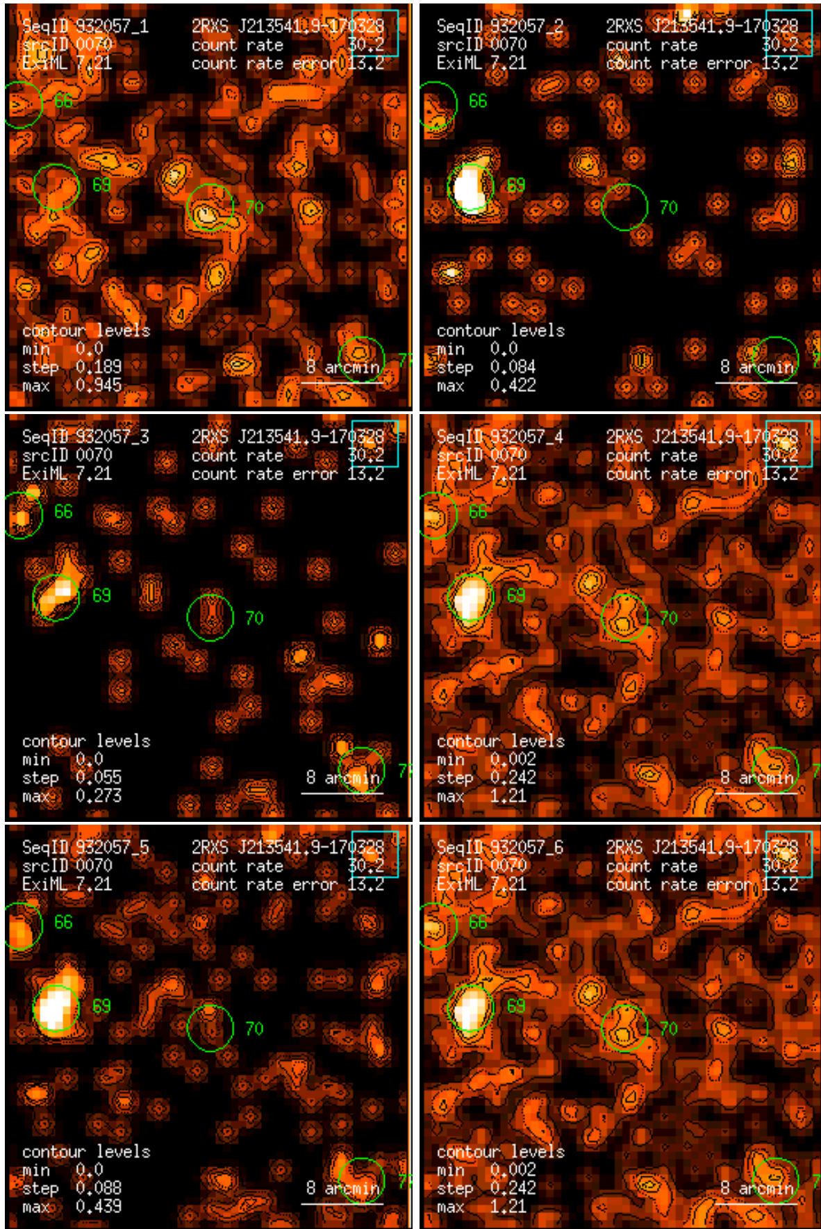
Figure 70: RASS 932057: detection 0070: band rate images, Gaussian filter: (1) PSPC channels 11 – 41, (2) 52 – 90, (3) 91 – 201, (4) 11 – 235, (5) 52 – 201, (6) 11 – 201. Broad band rates in counts/ks. Band rate contour levels in counts/ks/arcmin 2 .
