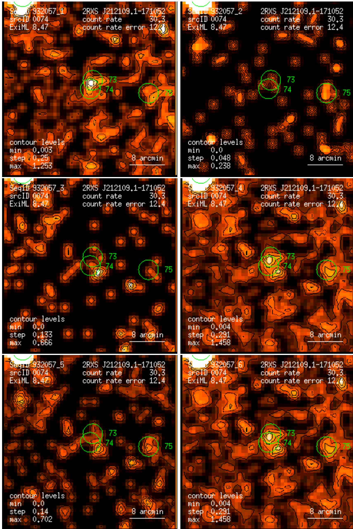
Figure 74: RASS 932057: detection 0074: band rate images, Gaussian filter: (1) PSPC channels 11 – 41, (2) 52 – 90, (3) 91 – 201, (4) 11 – 235, (5) 52 – 201, (6) 11 – 201. Broad band rates in counts/ks. Band rate contour levels in counts/ks/arcmin 2 .
