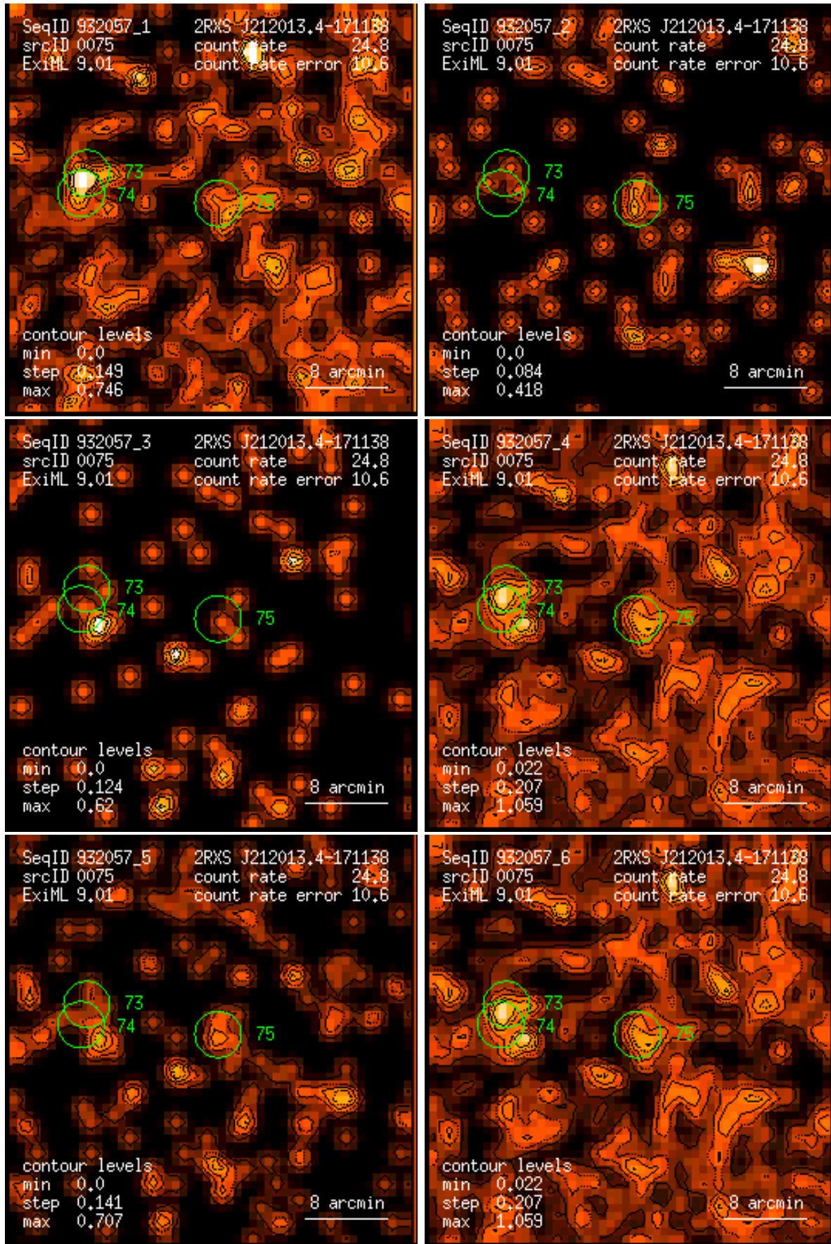
Figure 75: RASS 932057: detection 0075: band rate images, Gaussian filter: (1) PSPC channels 11 – 41, (2) 52 – 90, (3) 91 – 201, (4) 11 – 235, (5) 52 – 201, (6) 11 – 201. Broad band rates in counts/ks. Band rate contour levels in counts/ks/arcmin 2 .
