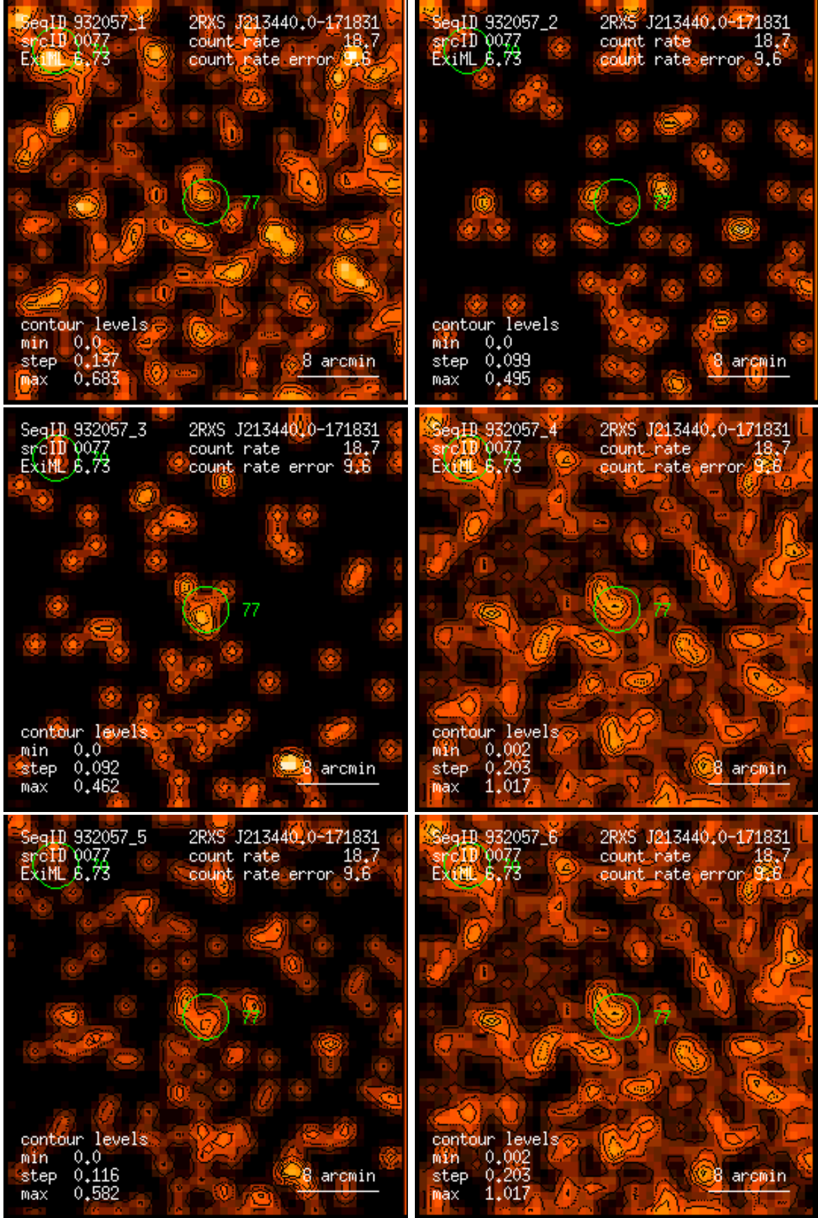
Figure 77: RASS 932057: detection 0077: band rate images, Gaussian filter: (1) PSPC channels 11 – 41, (2) 52 – 90, (3) 91 – 201, (4) 11 – 235, (5) 52 – 201, (6) 11 – 201. Broad band rates in counts/ks. Band rate contour levels in counts/ks/arcmin 2 .
