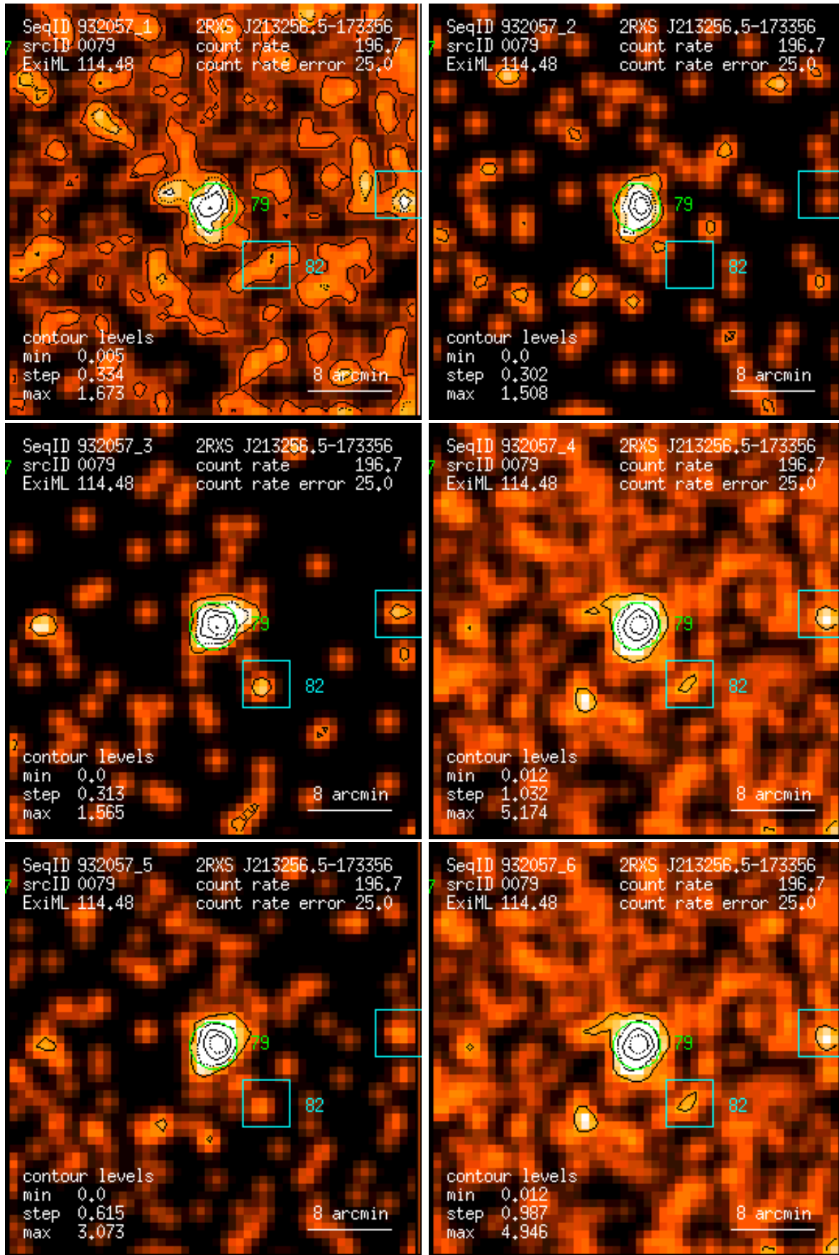
Figure 79: RASS 932057: detection 0079: band rate images, Gaussian filter: (1) PSPC channels 11 – 41, (2) 52 – 90, (3) 91 – 201, (4) 11 – 235, (5) 52 – 201, (6) 11 – 201. Broad band rates in counts/ks. Band rate contour levels in counts/ks/arcmin 2 .
