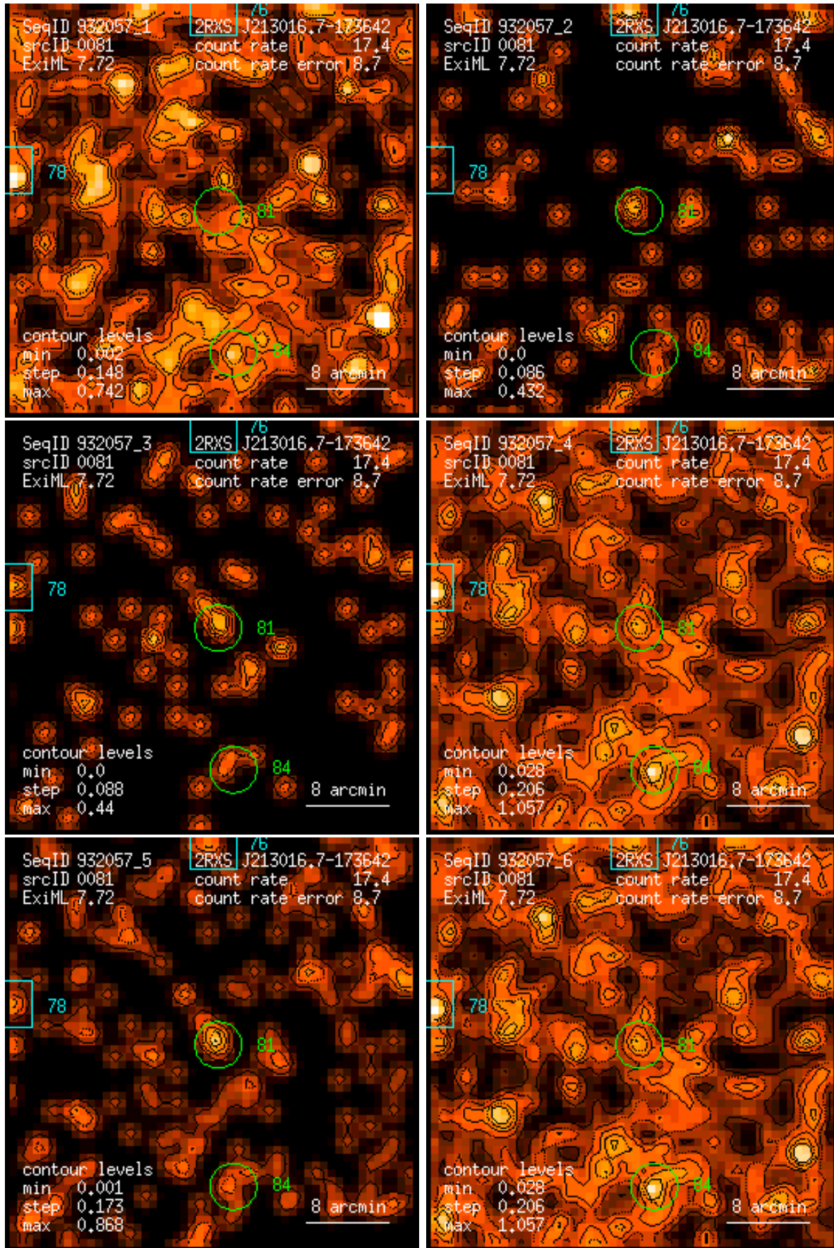
Figure 81: RASS 932057: detection 0081: band rate images, Gaussian filter: (1) PSPC channels 11 – 41, (2) 52 – 90, (3) 91 – 201, (4) 11 – 235, (5) 52 – 201, (6) 11 – 201. Broad band rates in counts/ks. Band rate contour levels in counts/ks/arcmin 2 .
