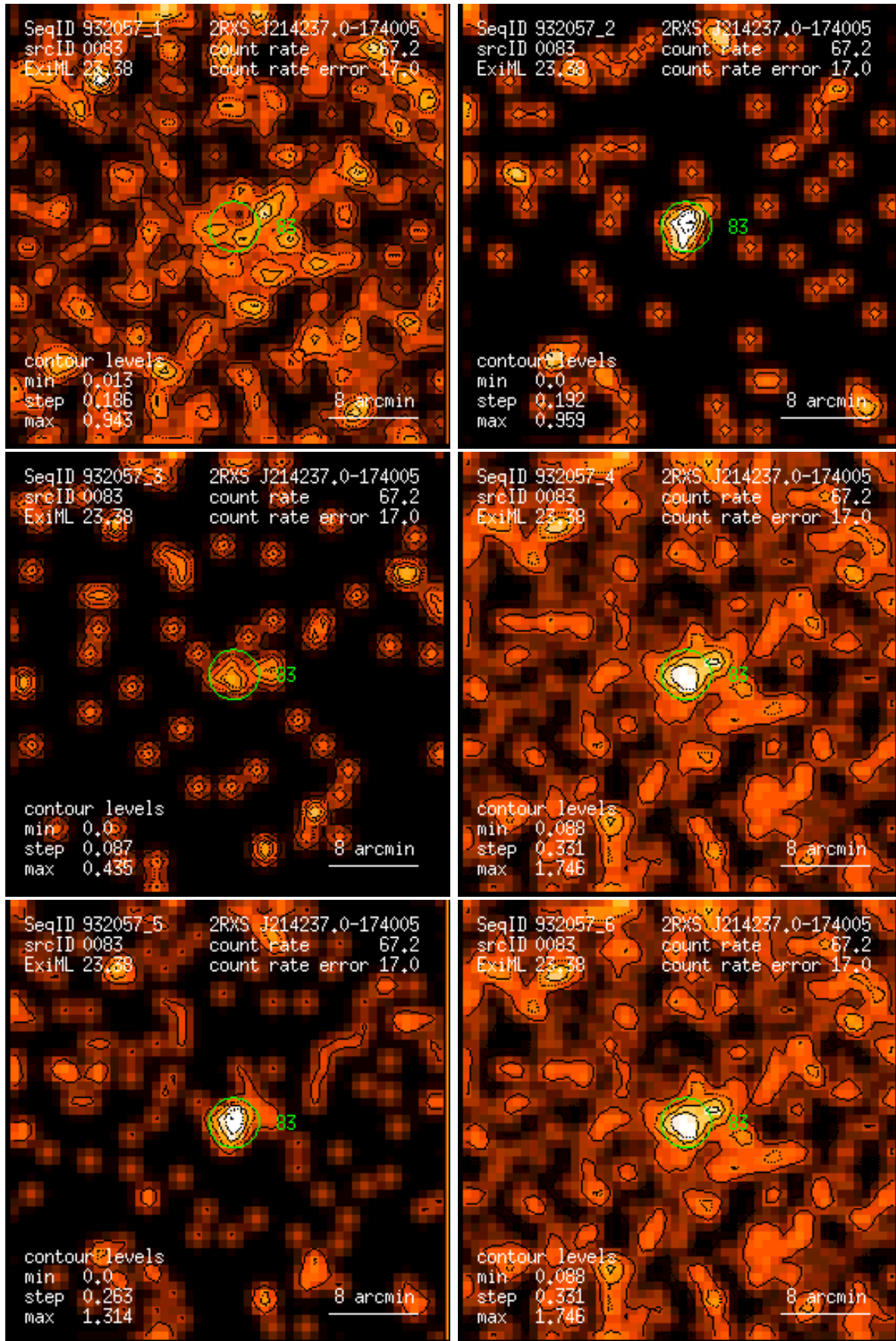
Figure 83: RASS 932057: detection 0083: band rate images, Gaussian filter: (1) PSPC channels 11 – 41, (2) 52 – 90, (3) 91 – 201, (4) 11 – 235, (5) 52 – 201, (6) 11 – 201. Broad band rates in counts/ks. Band rate contour levels in counts/ks/arcmin 2 .
