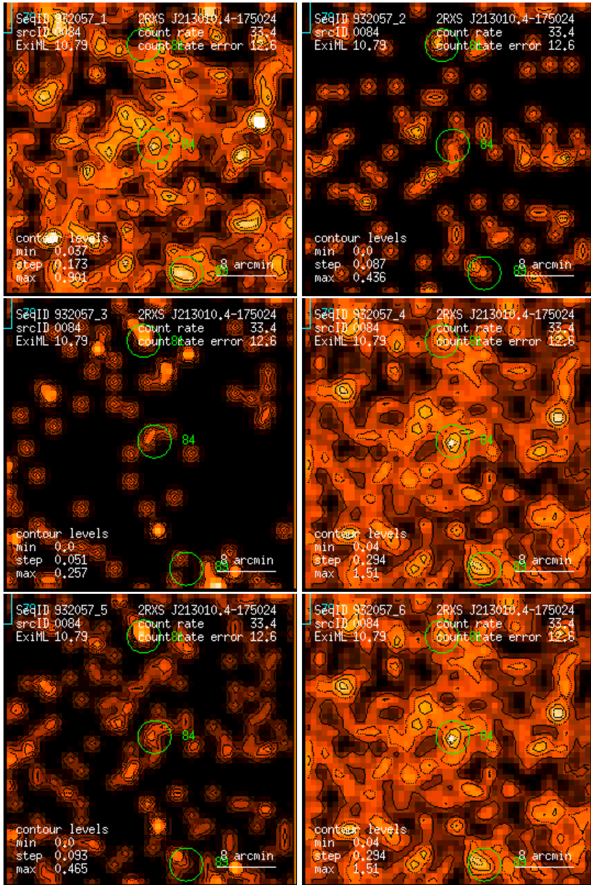
Figure 84: RASS 932057: detection 0084: band rate images, Gaussian filter: (1) PSPC channels 11 – 41, (2) 52 – 90, (3) 91 – 201, (4) 11 – 235, (5) 52 – 201, (6) 11 – 201. Broad band rates in counts/ks. Band rate contour levels in counts/ks/arcmin 2 .
