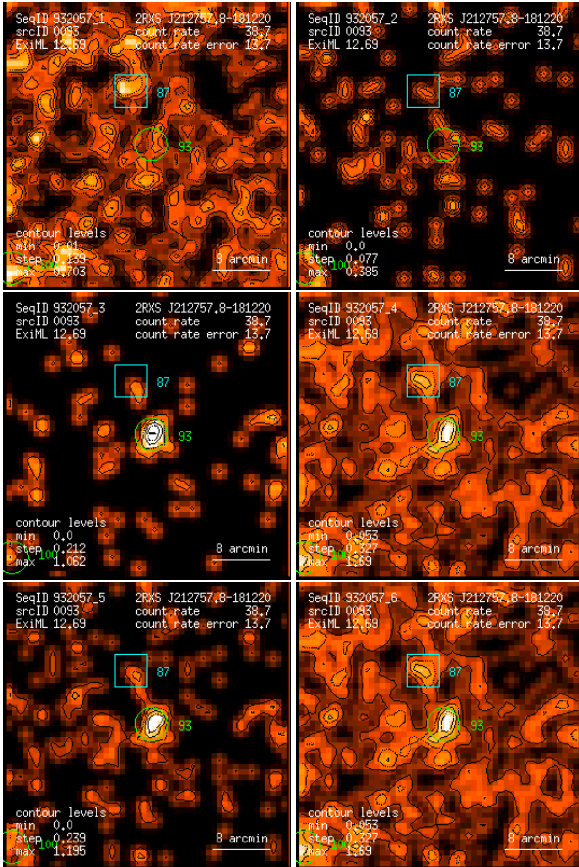
Figure 93: RASS 932057: detection 0093: band rate images, Gaussian filter: (1) PSPC channels 11 – 41, (2) 52 – 90, (3) 91 – 201, (4) 11 – 235, (5) 52 – 201, (6) 11 – 201. Broad band rates in counts/ks. Band rate contour levels in counts/ks/arcmin 2 .
