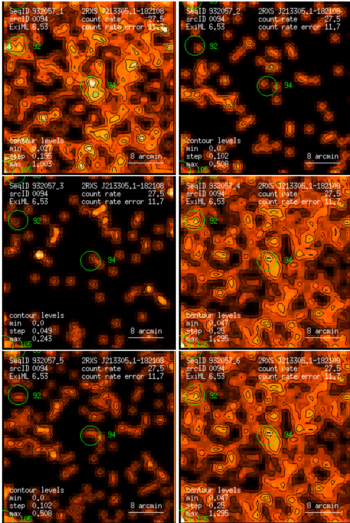
Figure 94: RASS 932057: detection 0094: band rate images, Gaussian filter: (1) PSPC channels 11 – 41, (2) 52 – 90, (3) 91 – 201, (4) 11 – 235, (5) 52 – 201, (6) 11 – 201. Broad band rates in counts/ks. Band rate contour levels in counts/ks/arcmin 2 .
