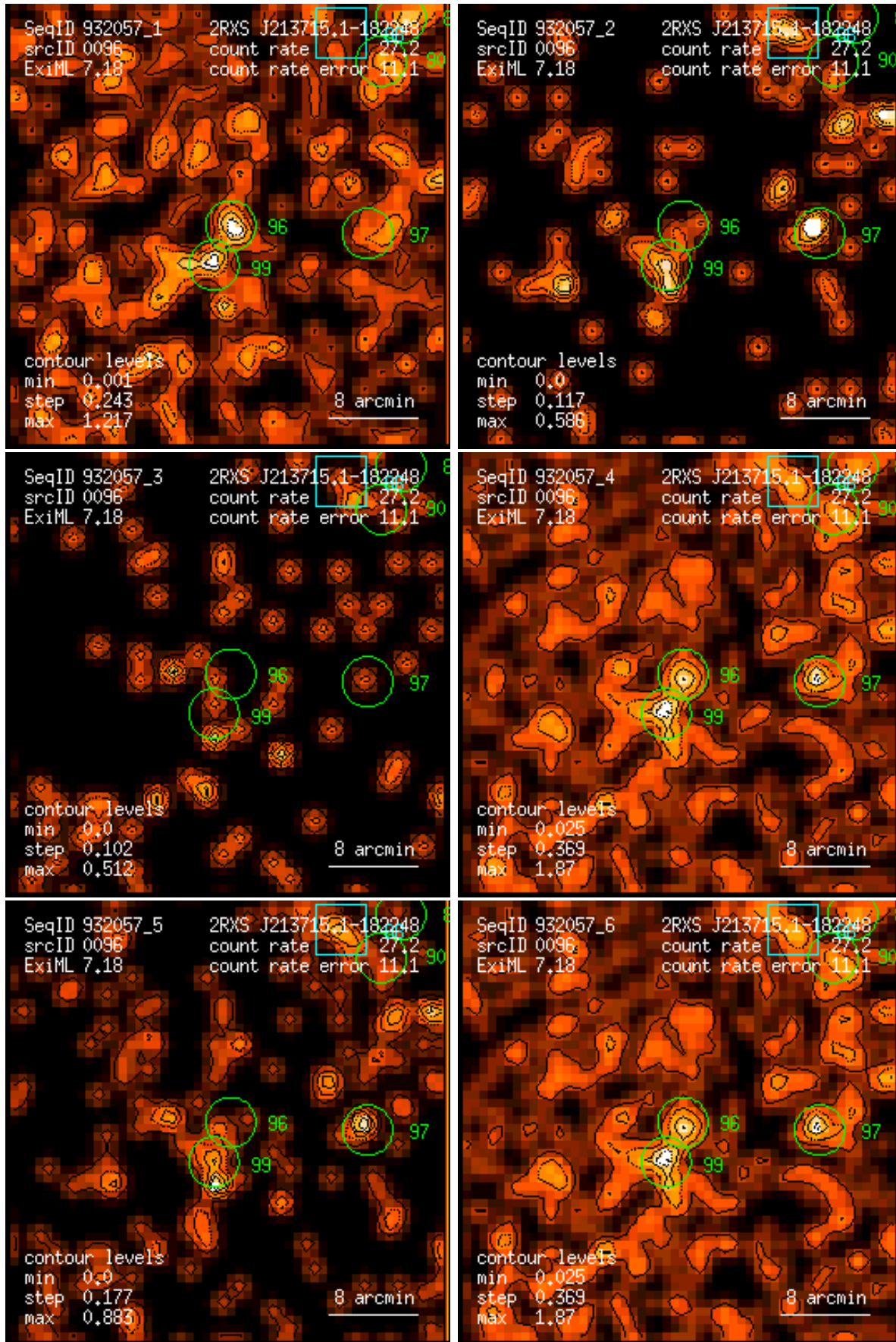
Figure 96: RASS 932057: detection 0096: band rate images, Gaussian filter: (1) PSPC channels 11 – 41, (2) 52 – 90, (3) 91 – 201, (4) 11 – 235, (5) 52 – 201, (6) 11 – 201. Broad band rates in counts/ks. Band rate contour levels in counts/ks/arcmin 2 .
