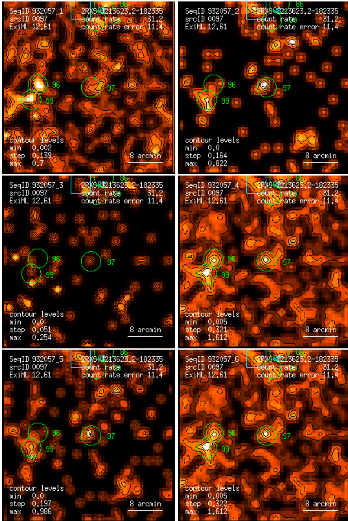
Figure 97: RASS 932057: detection 0097: band rate images, Gaussian filter: (1) PSPC channels 11 – 41, (2) 52 – 90, (3) 91 – 201, (4) 11 – 235, (5) 52 – 201, (6) 11 – 201. Broad band rates in counts/ks. Band rate contour levels in counts/ks/arcmin 2 .
