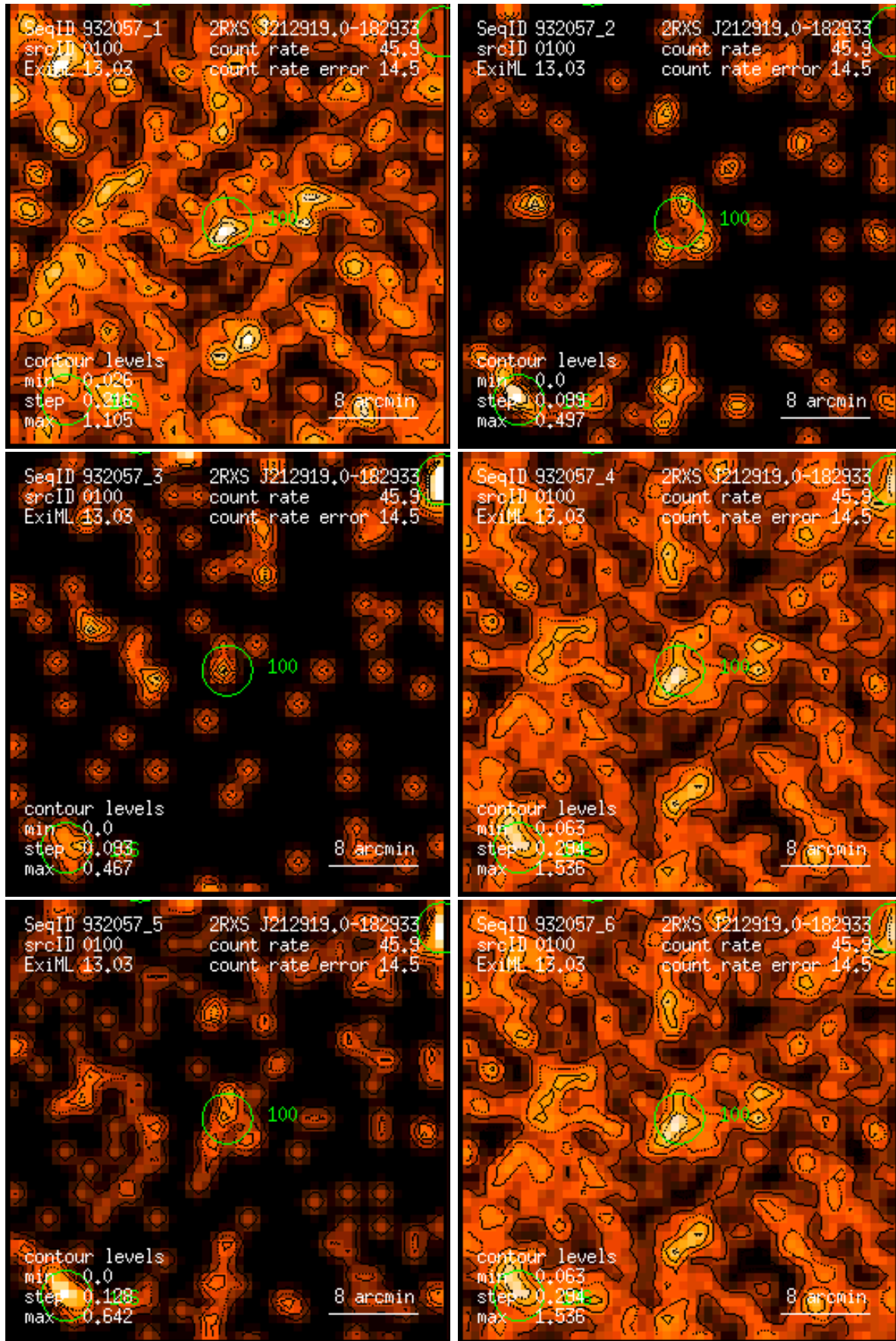
Figure 100: RASS 932057: detection 0100: band rate images, Gaussian filter: (1) PSPC channels 11 – 41, (2) 52 – 90, (3) 91 – 201, (4) 11 – 235, (5) 52 – 201, (6) 11 – 201. Broad band rates in counts/ks. Band rate contour levels in counts/ks/arcmin 2 .
