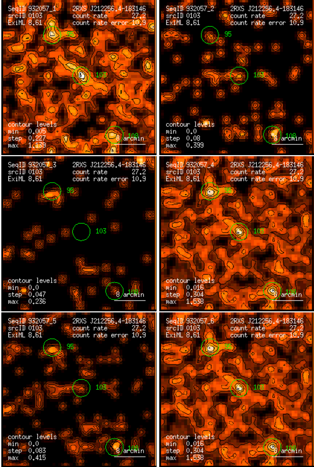
Figure 103: RASS 932057: detection 0103: band rate images, Gaussian filter: (1) PSPC channels 11 – 41, (2) 52 – 90, (3) 91 – 201, (4) 11 – 235, (5) 52 – 201, (6) 11 – 201. Broad band rates in counts/ks. Band rate contour levels in counts/ks/arcmin 2 .
