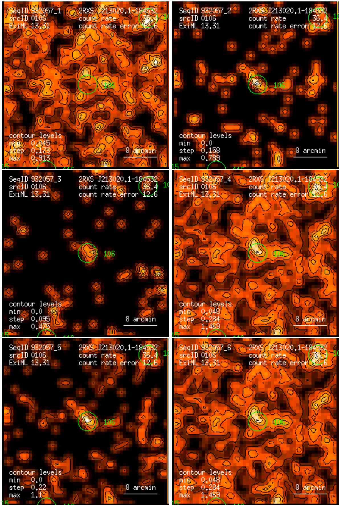
Figure 106: RASS 932057: detection 0106: band rate images, Gaussian filter: (1) PSPC channels 11 – 41, (2) 52 – 90, (3) 91 – 201, (4) 11 – 235, (5) 52 – 201, (6) 11 – 201. Broad band rates in counts/ks. Band rate contour levels in counts/ks/arcmin 2 .
