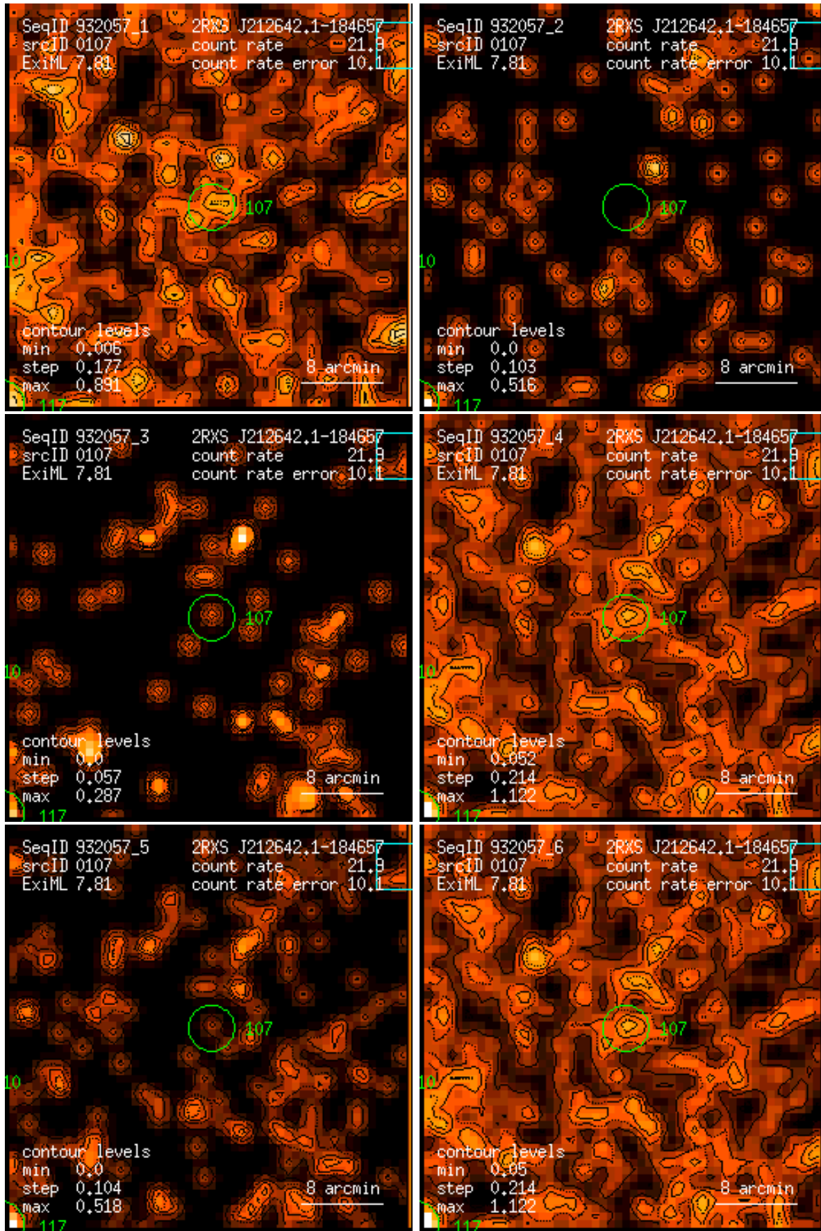
Figure 107: RASS 932057: detection 0107: band rate images, Gaussian filter: (1) PSPC channels 11 – 41, (2) 52 – 90, (3) 91 – 201, (4) 11 – 235, (5) 52 – 201, (6) 11 – 201. Broad band rates in counts/ks. Band rate contour levels in counts/ks/arcmin 2 .
