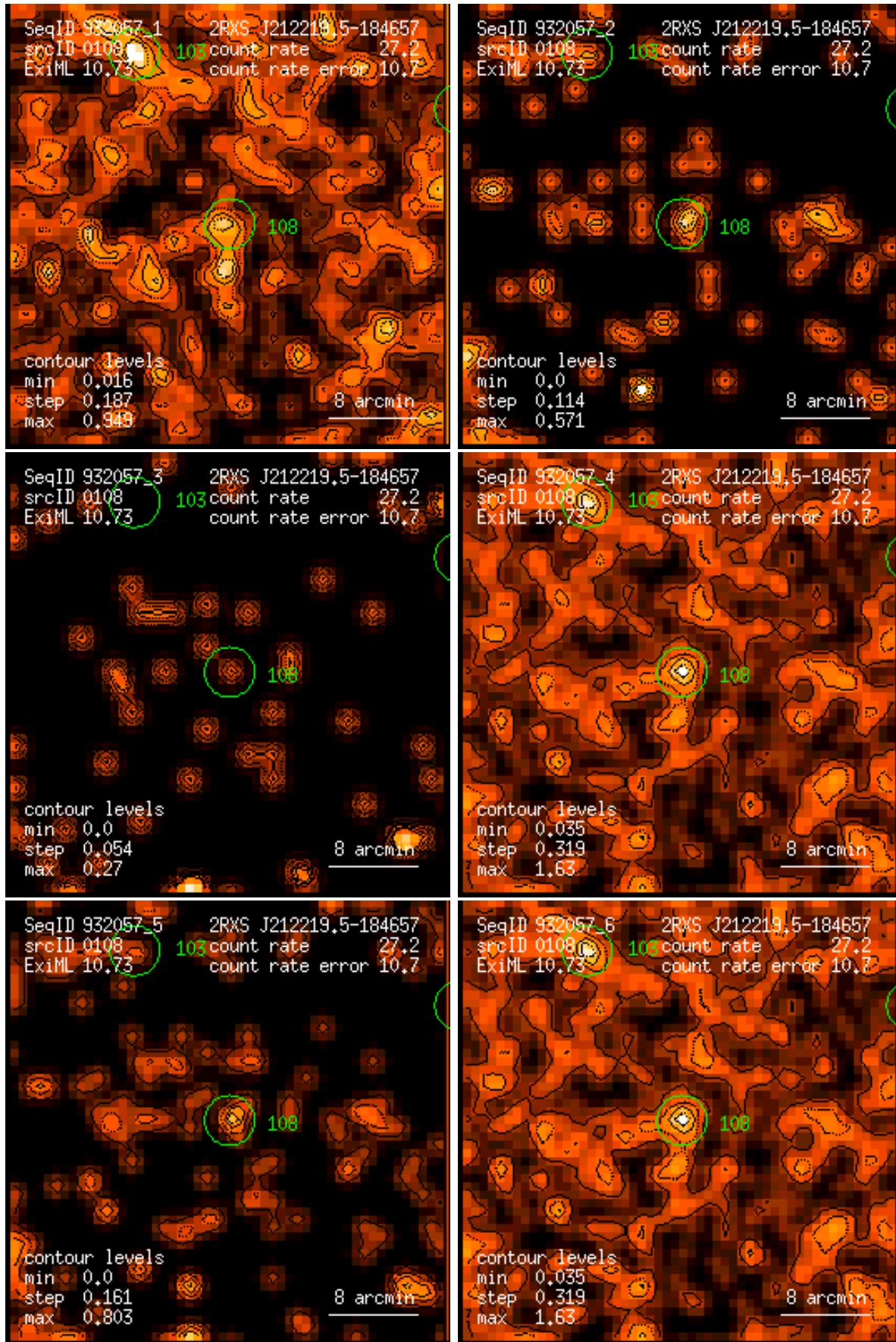
Figure 108: RASS 932057: detection 0108: band rate images, Gaussian filter: (1) PSPC channels 11 – 41, (2) 52 – 90, (3) 91 – 201, (4) 11 – 235, (5) 52 – 201, (6) 11 – 201. Broad band rates in counts/ks. Band rate contour levels in counts/ks/arcmin 2 .
