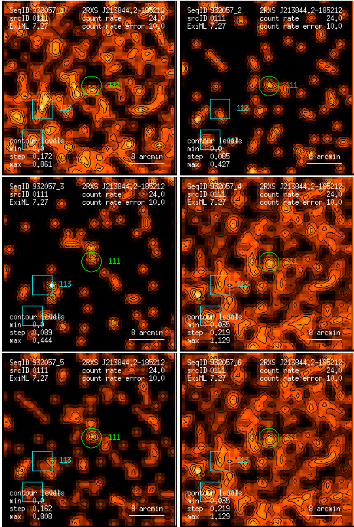
Figure 111: RASS 932057: detection 0111: band rate images, Gaussian filter: (1) PSPC channels 11 – 41, (2) 52 – 90, (3) 91 – 201, (4) 11 – 235, (5) 52 – 201, (6) 11 – 201. Broad band rates in counts/ks. Band rate contour levels in counts/ks/arcmin 2 .
