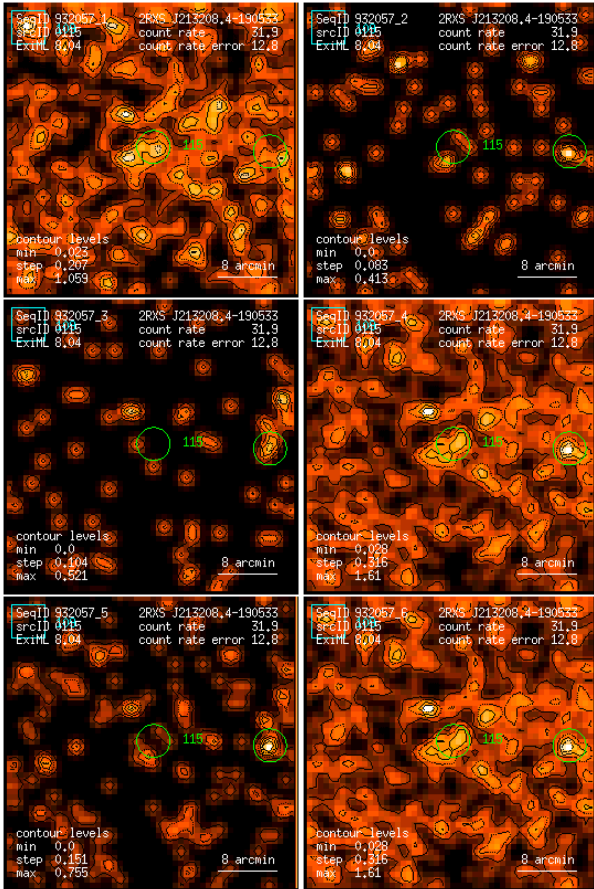
Figure 115: RASS 932057: detection 0115: band rate images, Gaussian filter: (1) PSPC channels 11 – 41, (2) 52 – 90, (3) 91 – 201, (4) 11 – 235, (5) 52 – 201, (6) 11 – 201. Broad band rates in counts/ks. Band rate contour levels in counts/ks/arcmin 2 .
