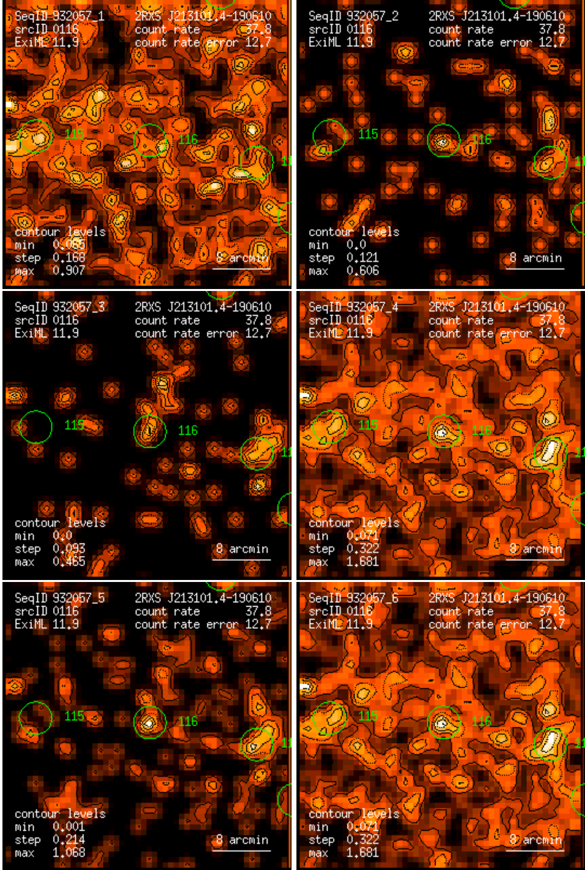
Figure 116: RASS 932057: detection 0116: band rate images, Gaussian filter: (1) PSPC channels 11 – 41, (2) 52 – 90, (3) 91 – 201, (4) 11 – 235, (5) 52 – 201, (6) 11 – 201. Broad band rates in counts/ks. Band rate contour levels in counts/ks/arcmin 2 .
