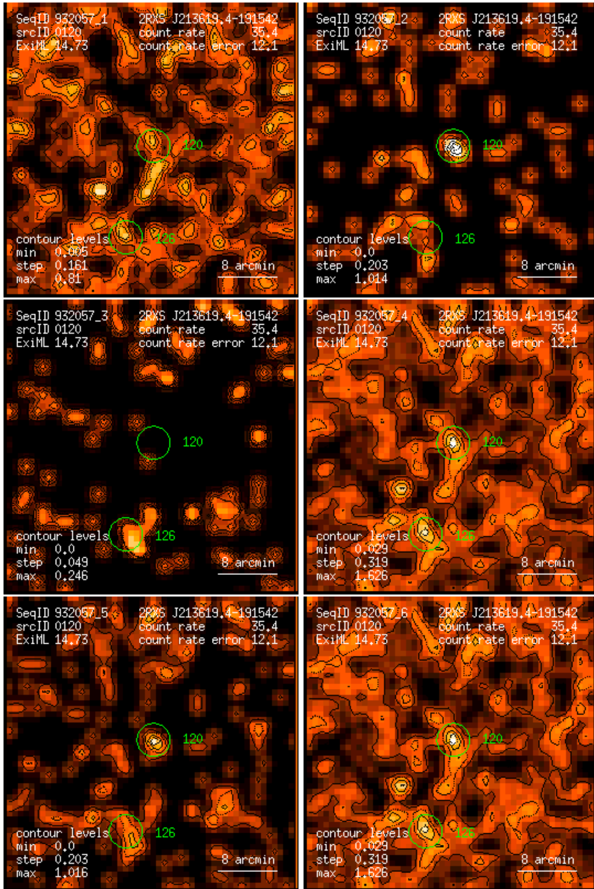
Figure 120: RASS 932057: detection 0120: band rate images, Gaussian filter: (1) PSPC channels 11 – 41, (2) 52 – 90, (3) 91 – 201, (4) 11 – 235, (5) 52 – 201, (6) 11 – 201. Broad band rates in counts/ks. Band rate contour levels in counts/ks/arcmin 2 .
