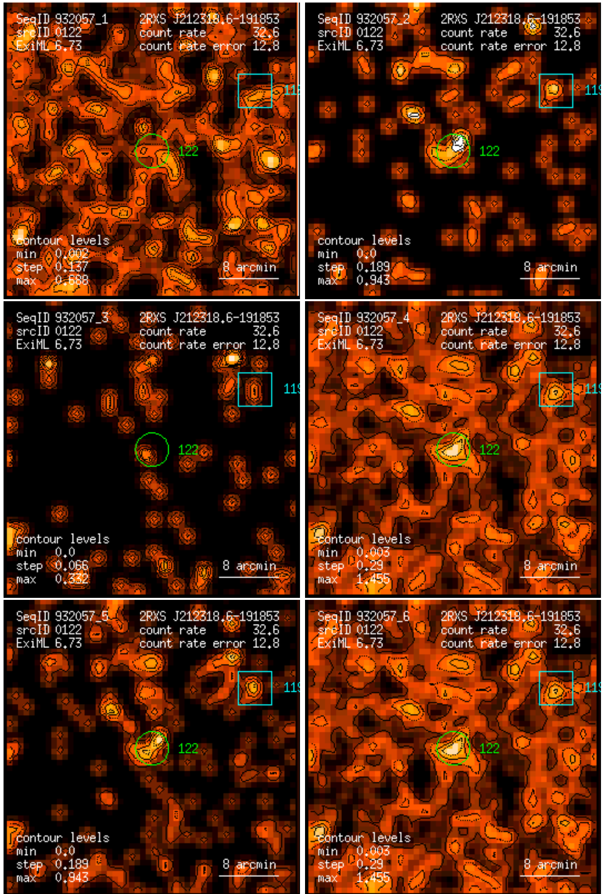
Figure 122: RASS 932057: detection 0122: band rate images, Gaussian filter: (1) PSPC channels 11 – 41, (2) 52 – 90, (3) 91 – 201, (4) 11 – 235, (5) 52 – 201, (6) 11 – 201. Broad band rates in counts/ks. Band rate contour levels in counts/ks/arcmin 2 .
