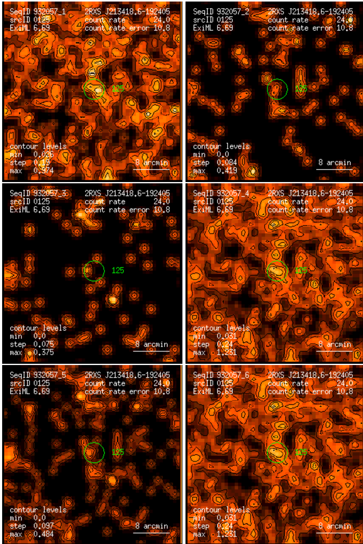
Figure 125: RASS 932057: detection 0125: band rate images, Gaussian filter: (1) PSPC channels 11 – 41, (2) 52 – 90, (3) 91 – 201, (4) 11 – 235, (5) 52 – 201, (6) 11 – 201. Broad band rates in counts/ks. Band rate contour levels in counts/ks/arcmin 2 .
