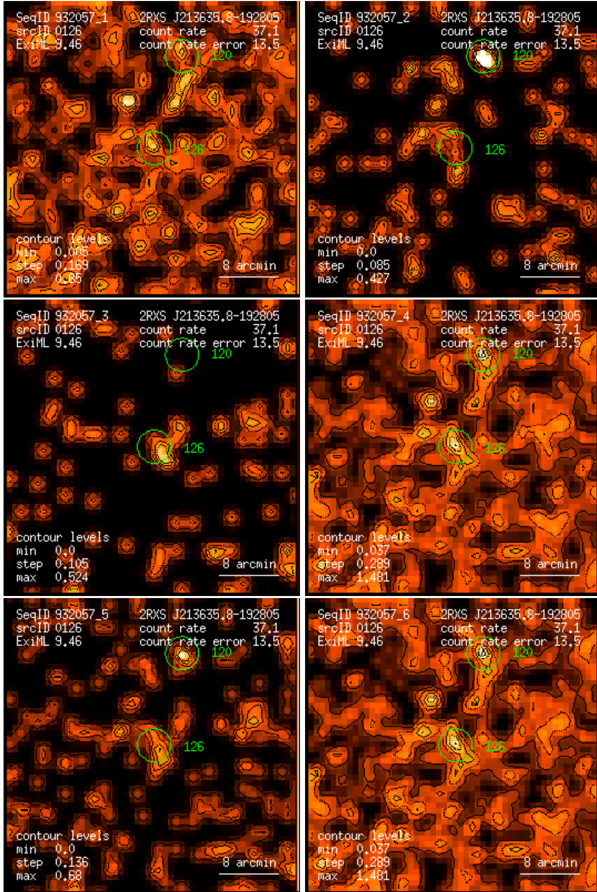
Figure 126: RASS 932057: detection 0126: band rate images, Gaussian filter: (1) PSPC channels 11 – 41, (2) 52 – 90, (3) 91 – 201, (4) 11 – 235, (5) 52 – 201, (6) 11 – 201. Broad band rates in counts/ks. Band rate contour levels in counts/ks/arcmin 2 .
