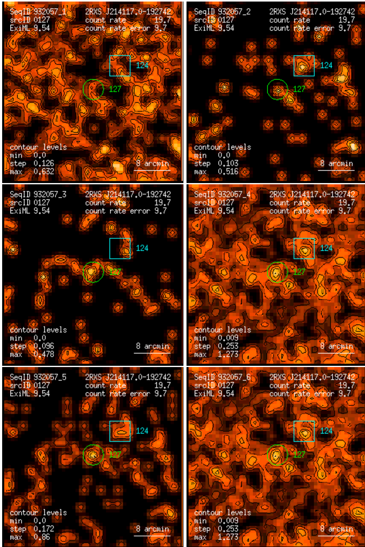
Figure 127: RASS 932057: detection 0127: band rate images, Gaussian filter: (1) PSPC channels 11 – 41, (2) 52 – 90, (3) 91 – 201, (4) 11 – 235, (5) 52 – 201, (6) 11 – 201. Broad band rates in counts/ks. Band rate contour levels in counts/ks/arcmin 2 .
