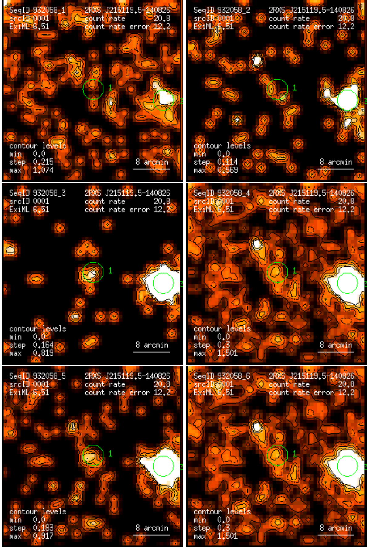
Figure 1: RASS 932058: detection 0001: band rate images, Gaussian filter: (1) PSPC channels 11 – 41, (2) 52 – 90, (3) 91 – 201, (4) 11 – 235, (5) 52 – 201, (6) 11 – 201. Broad band rates in counts/ks. Band rate contour levels in counts/ks/arcmin 2 .
