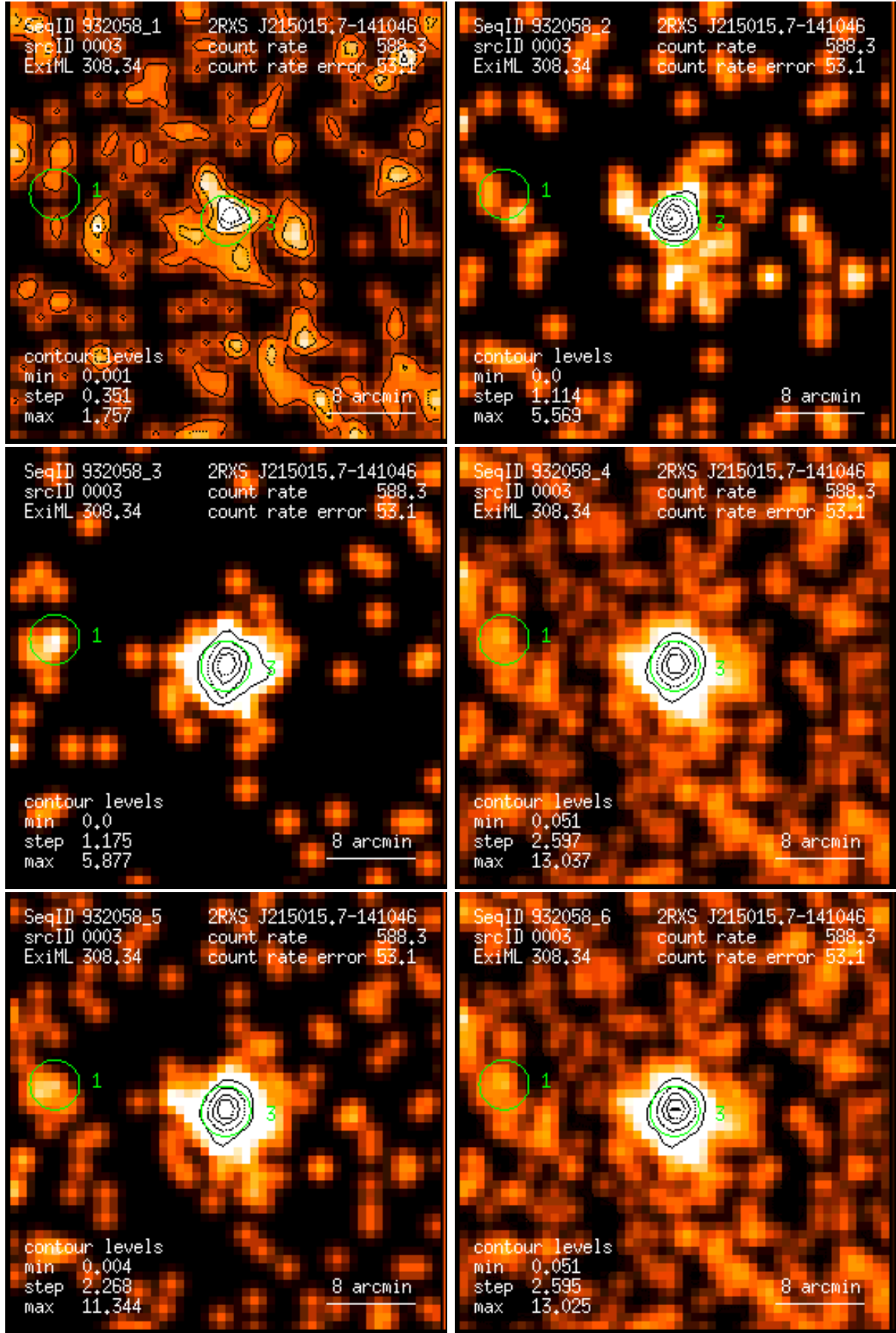
Figure 3: RASS 932058: detection 0003: band rate images, Gaussian filter: (1) PSPC channels 11 – 41, (2) 52 – 90, (3) 91 – 201, (4) 11 – 235, (5) 52 – 201, (6) 11 – 201. Broad band rates in counts/ks. Band rate contour levels in counts/ks/arcmin 2 .
