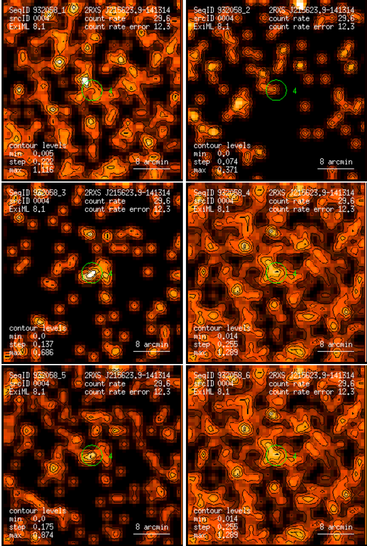
Figure 4: RASS 932058: detection 0004: band rate images, Gaussian filter: (1) PSPC channels 11 – 41, (2) 52 – 90, (3) 91 – 201, (4) 11 – 235, (5) 52 – 201, (6) 11 – 201. Broad band rates in counts/ks. Band rate contour levels in counts/ks/arcmin 2 .
