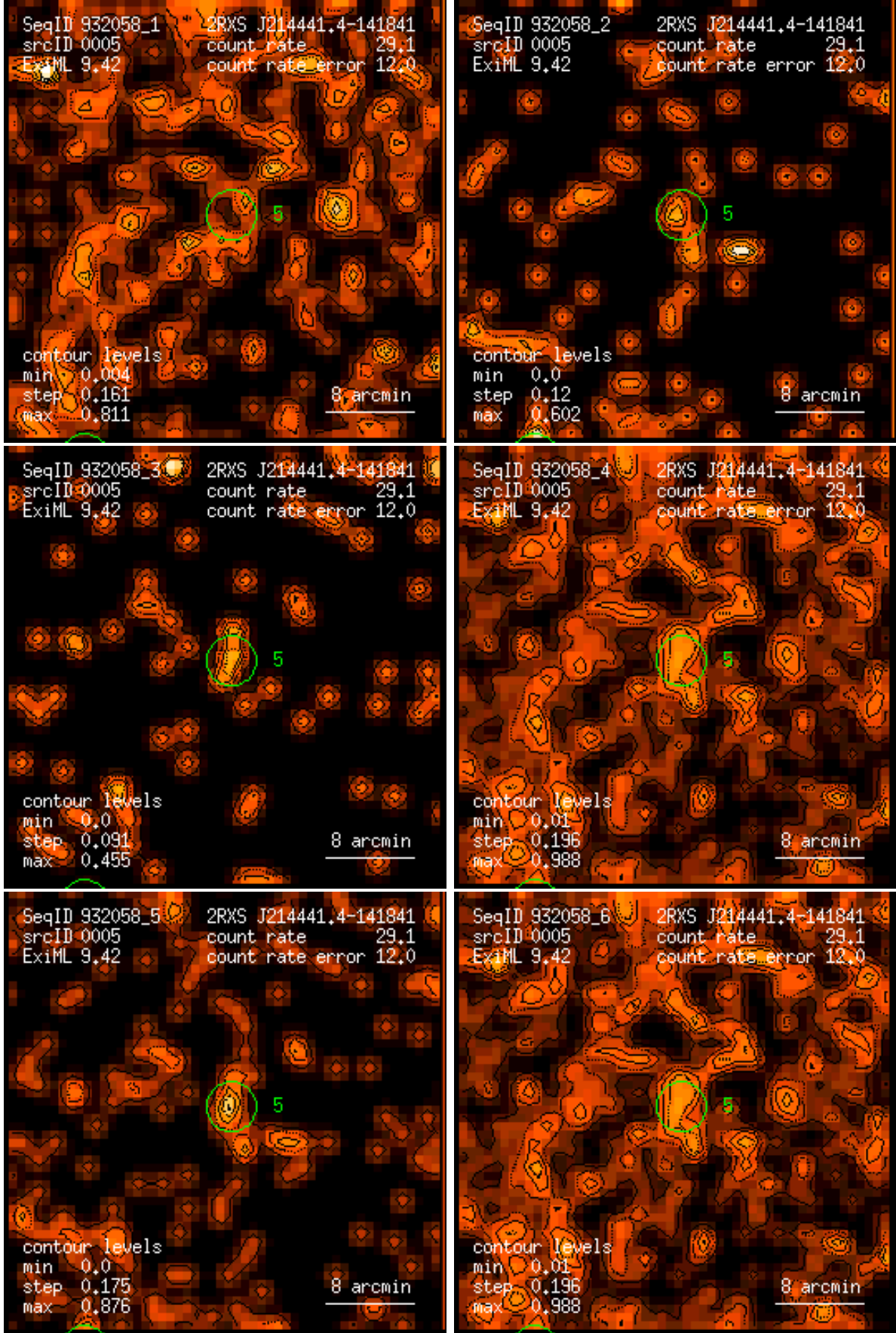
Figure 5: RASS 932058: detection 0005: band rate images, Gaussian filter: (1) PSPC channels 11 – 41, (2) 52 – 90, (3) 91 – 201, (4) 11 – 235, (5) 52 – 201, (6) 11 – 201. Broad band rates in counts/ks. Band rate contour levels in counts/ks/arcmin 2 .
