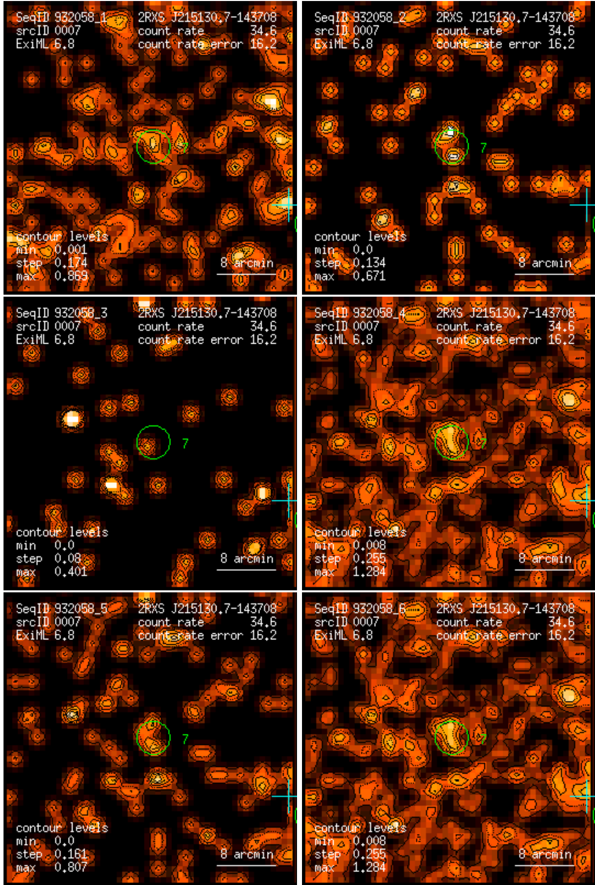
Figure 7: RASS 932058: detection 0007: band rate images, Gaussian filter: (1) PSPC channels 11 – 41, (2) 52 – 90, (3) 91 – 201, (4) 11 – 235, (5) 52 – 201, (6) 11 – 201. Broad band rates in counts/ks. Band rate contour levels in counts/ks/arcmin 2 .
