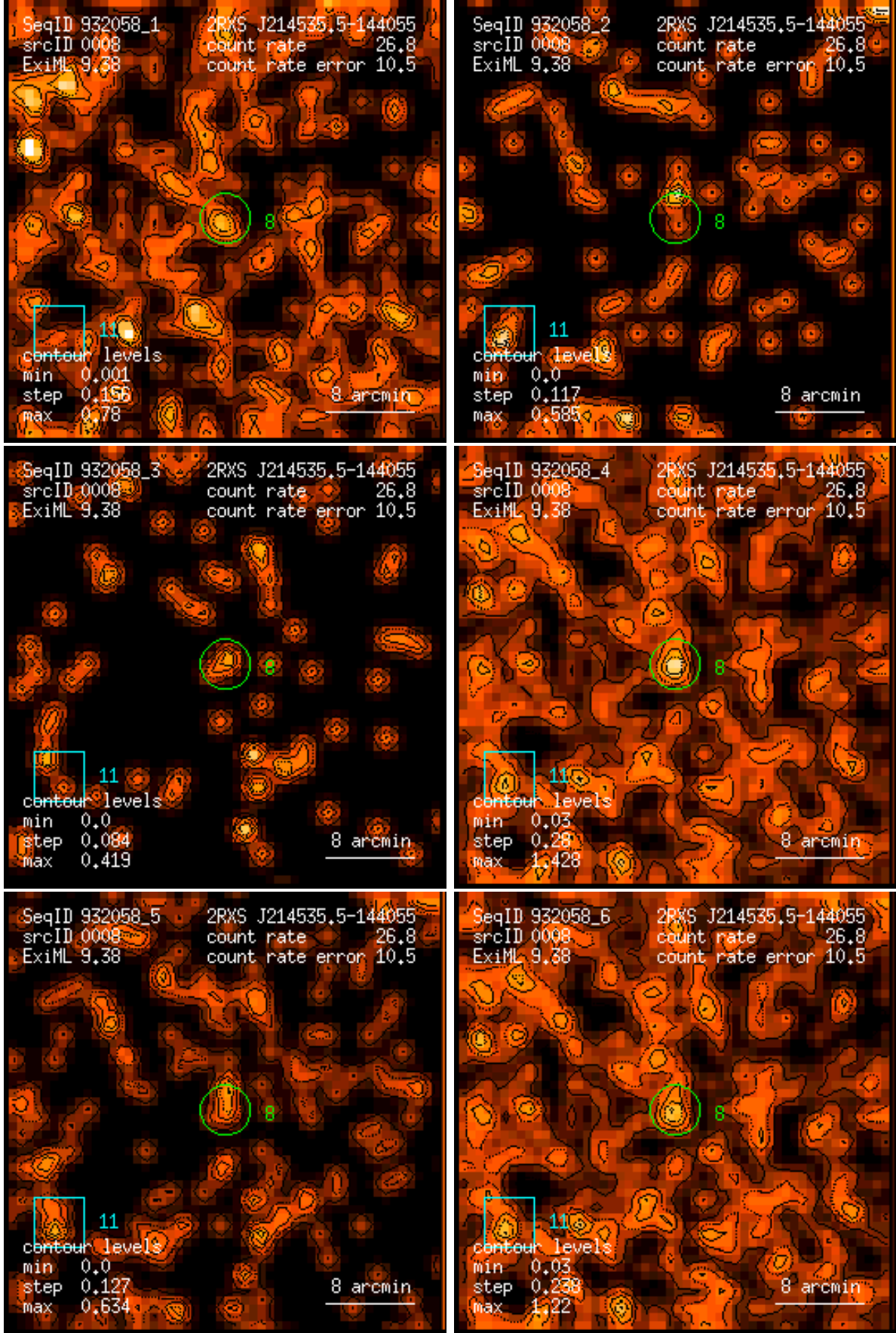
Figure 8: RASS 932058: detection 0008: band rate images, Gaussian filter: (1) PSPC channels 11 – 41, (2) 52 – 90, (3) 91 – 201, (4) 11 – 235, (5) 52 – 201, (6) 11 – 201. Broad band rates in counts/ks. Band rate contour levels in counts/ks/arcmin 2 .
