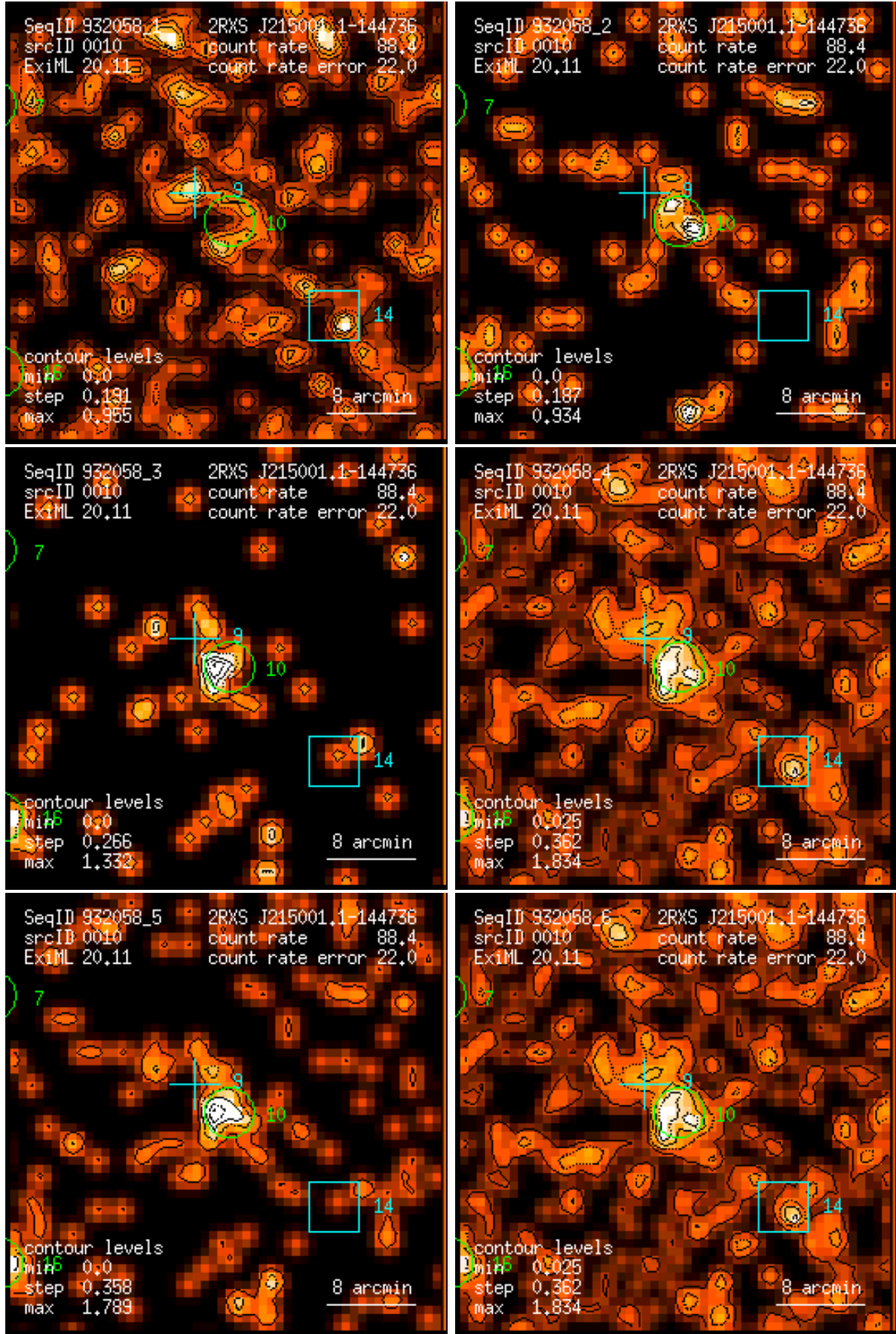
Figure 10: RASS 932058: detection 0010: band rate images, Gaussian filter: (1) PSPC channels 11 – 41, (2) 52 – 90, (3) 91 – 201, (4) 11 – 235, (5) 52 – 201, (6) 11 – 201. Broad band rates in counts/ks. Band rate contour levels in counts/ks/arcmin 2 .
