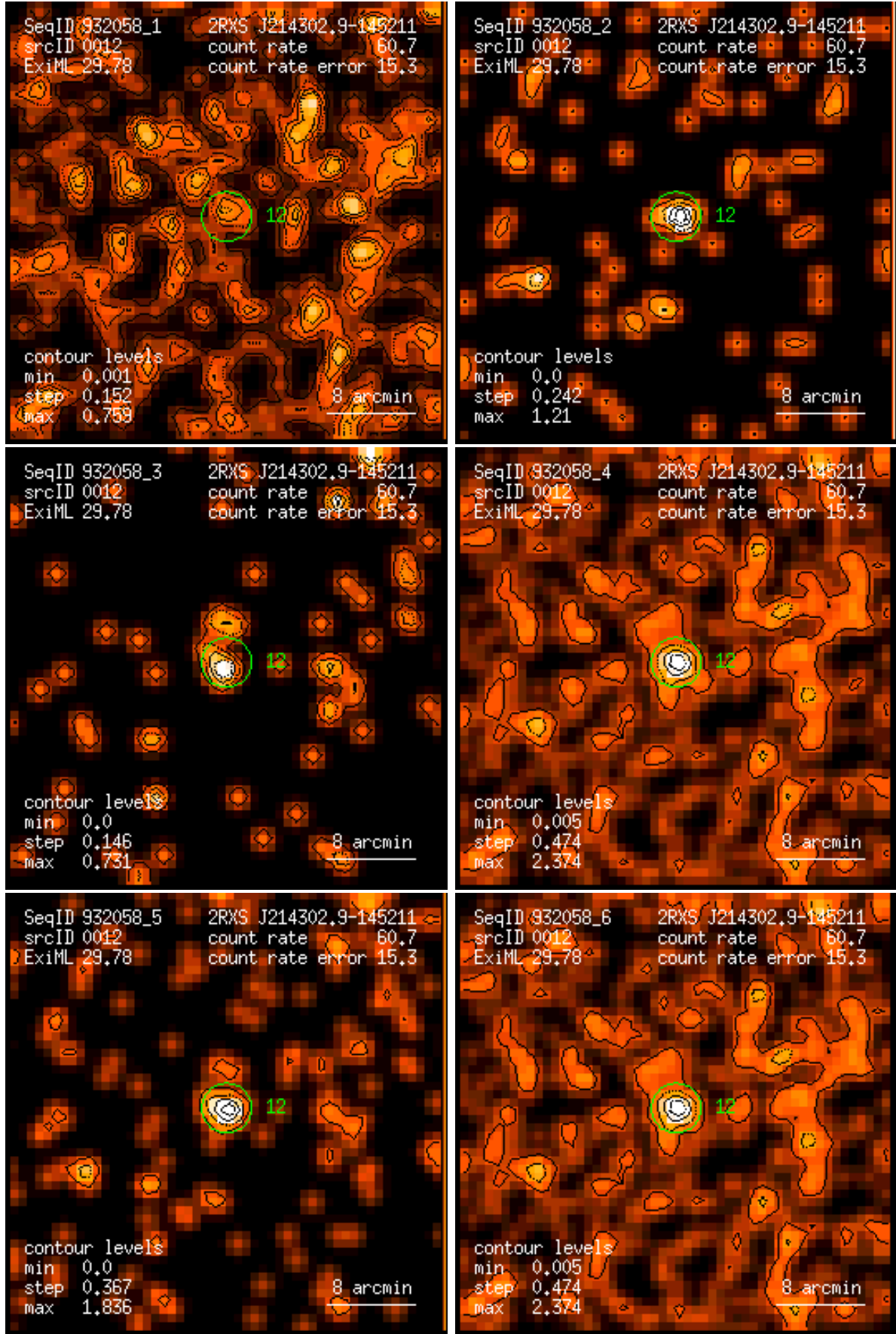
Figure 12: RASS 932058: detection 0012: band rate images, Gaussian filter: (1) PSPC channels 11 – 41, (2) 52 – 90, (3) 91 – 201, (4) 11 – 235, (5) 52 – 201, (6) 11 – 201. Broad band rates in counts/ks. Band rate contour levels in counts/ks/arcmin 2 .
