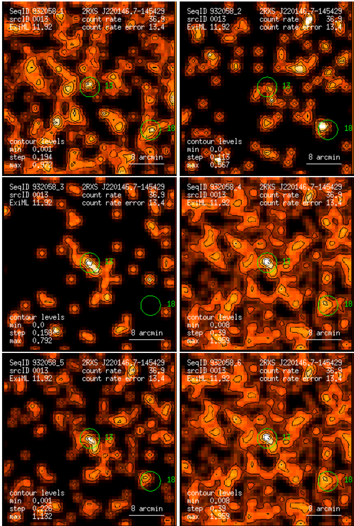
Figure 13: RASS 932058: detection 0013: band rate images, Gaussian filter: (1) PSPC channels 11 – 41, (2) 52 – 90, (3) 91 – 201, (4) 11 – 235, (5) 52 – 201, (6) 11 – 201. Broad band rates in counts/ks. Band rate contour levels in counts/ks/arcmin 2 .
