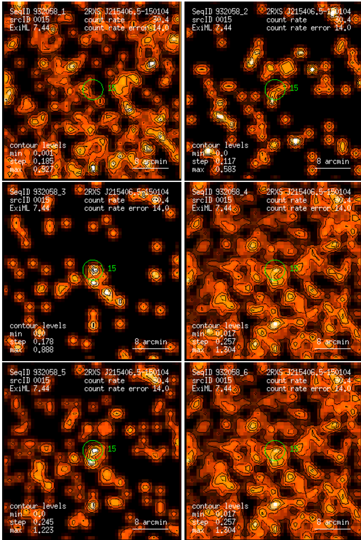
Figure 15: RASS 932058: detection 0015: band rate images, Gaussian filter: (1) PSPC channels 11 – 41, (2) 52 – 90, (3) 91 – 201, (4) 11 – 235, (5) 52 – 201, (6) 11 – 201. Broad band rates in counts/ks. Band rate contour levels in counts/ks/arcmin 2 .
