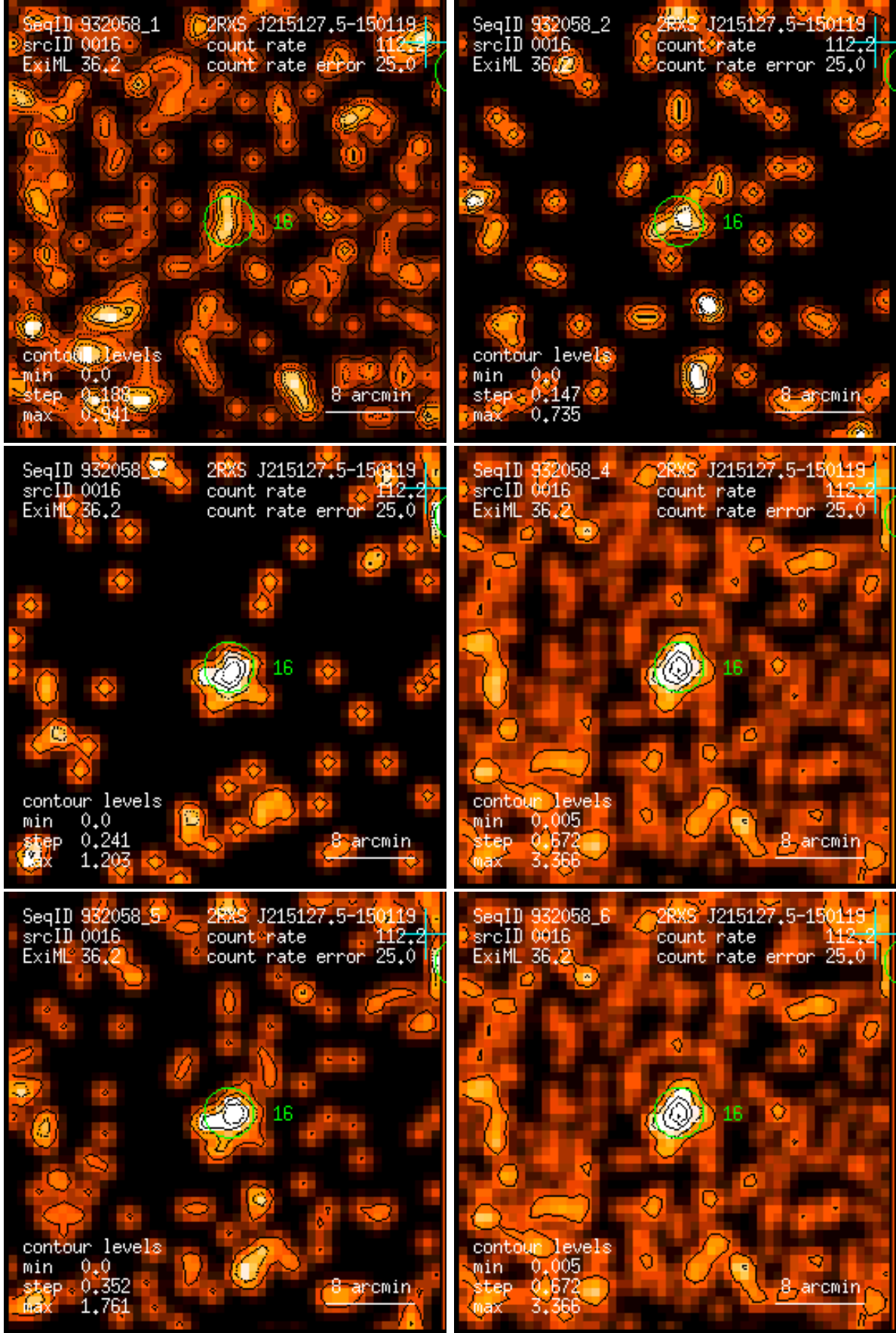
Figure 16: RASS 932058: detection 0016: band rate images, Gaussian filter: (1) PSPC channels 11 – 41, (2) 52 – 90, (3) 91 – 201, (4) 11 – 235, (5) 52 – 201, (6) 11 – 201. Broad band rates in counts/ks. Band rate contour levels in counts/ks/arcmin 2 .
