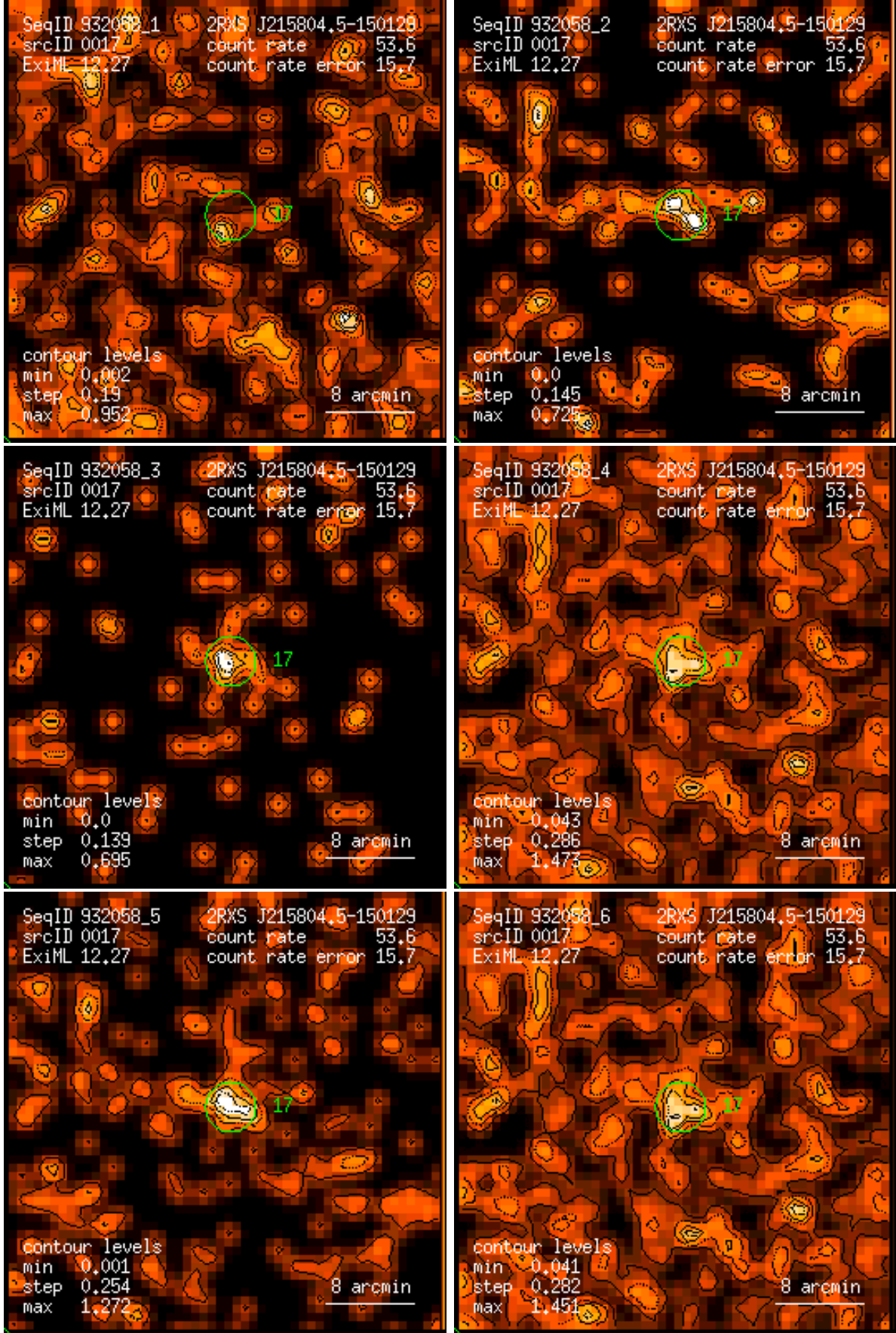
Figure 17: RASS 932058: detection 0017: band rate images, Gaussian filter: (1) PSPC channels 11 – 41, (2) 52 – 90, (3) 91 – 201, (4) 11 – 235, (5) 52 – 201, (6) 11 – 201. Broad band rates in counts/ks. Band rate contour levels in counts/ks/arcmin 2 .
