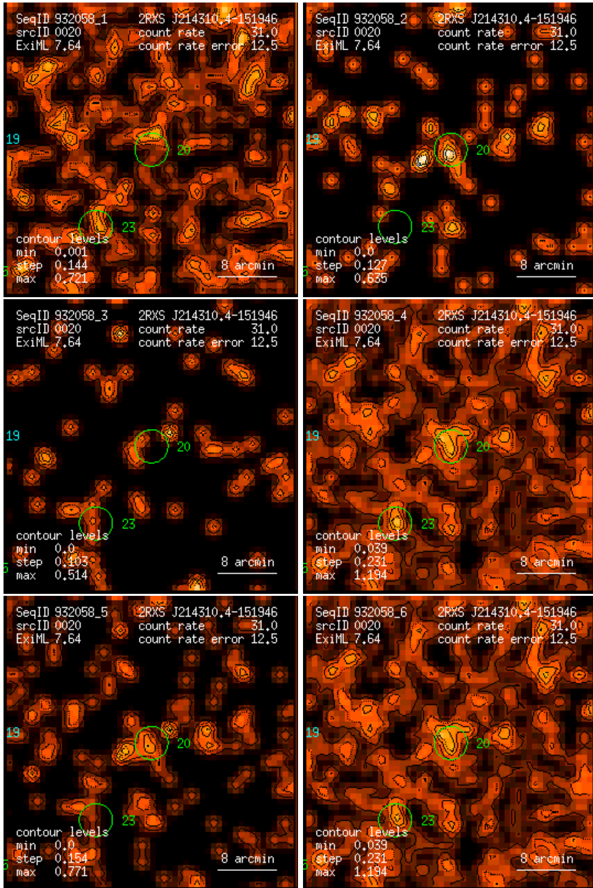
Figure 20: RASS 932058: detection 0020: band rate images, Gaussian filter: (1) PSPC channels 11 – 41, (2) 52 – 90, (3) 91 – 201, (4) 11 – 235, (5) 52 – 201, (6) 11 – 201. Broad band rates in counts/ks. Band rate contour levels in counts/ks/arcmin 2 .
