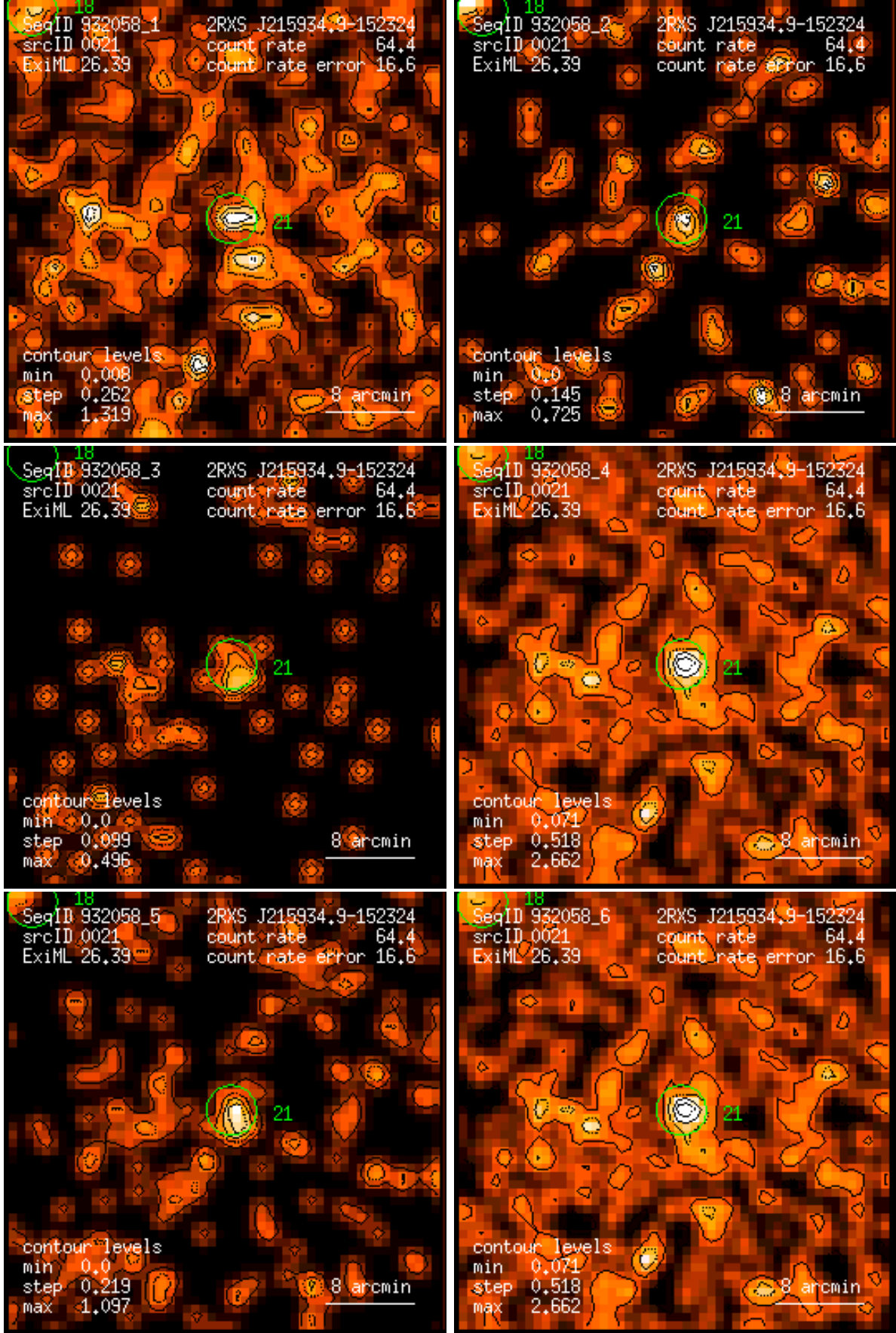
Figure 21: RASS 932058: detection 0021: band rate images, Gaussian filter: (1) PSPC channels 11 – 41, (2) 52 – 90, (3) 91 – 201, (4) 11 – 235, (5) 52 – 201, (6) 11 – 201. Broad band rates in counts/ks. Band rate contour levels in counts/ks/arcmin 2 .
