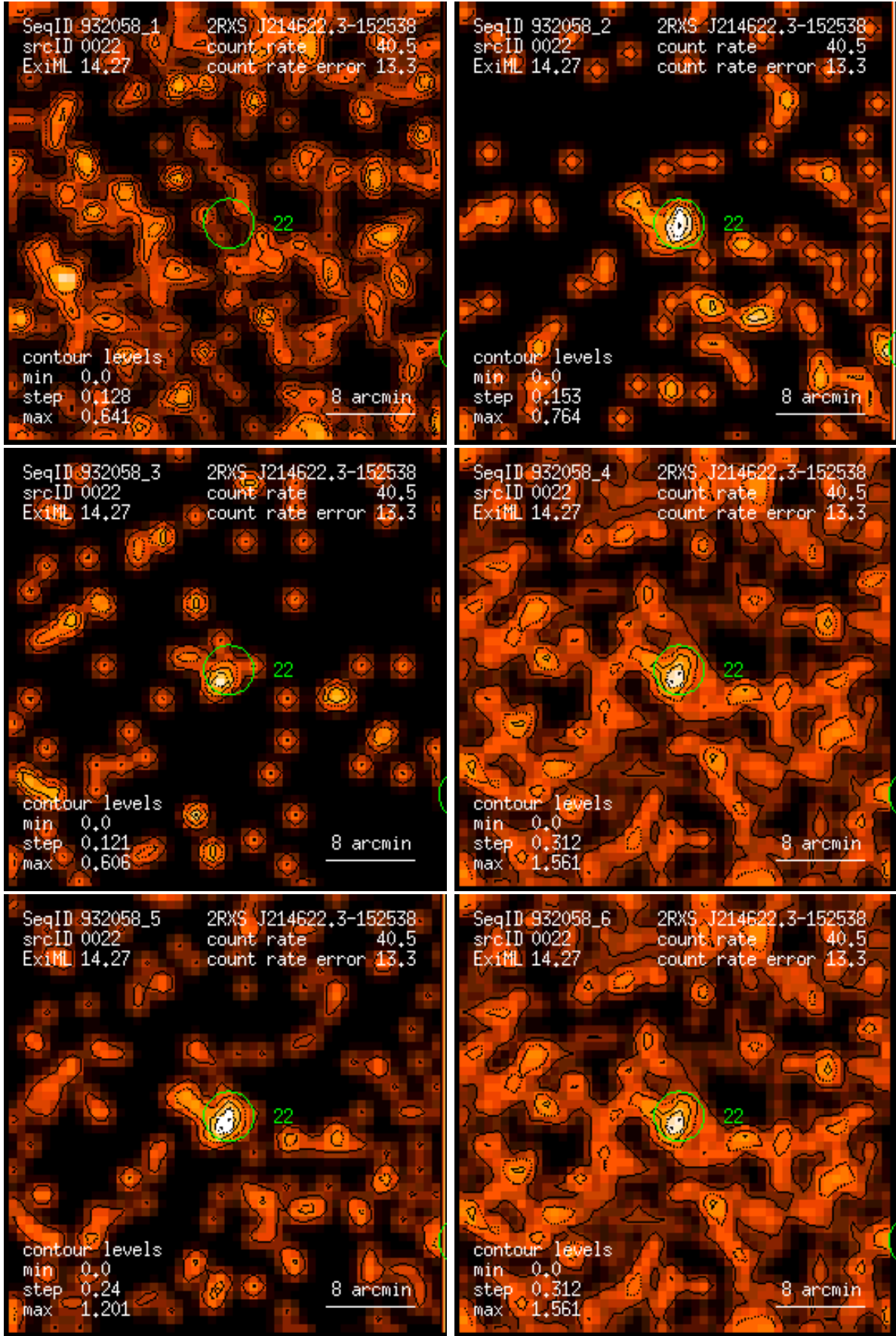
Figure 22: RASS 932058: detection 0022: band rate images, Gaussian filter: (1) PSPC channels 11 – 41, (2) 52 – 90, (3) 91 – 201, (4) 11 – 235, (5) 52 – 201, (6) 11 – 201. Broad band rates in counts/ks. Band rate contour levels in counts/ks/arcmin 2 .
