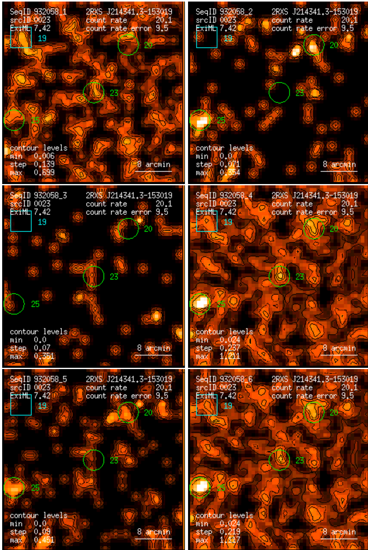
Figure 23: RASS 932058: detection 0023: band rate images, Gaussian filter: (1) PSPC channels 11 – 41, (2) 52 – 90, (3) 91 – 201, (4) 11 – 235, (5) 52 – 201, (6) 11 – 201. Broad band rates in counts/ks. Band rate contour levels in counts/ks/arcmin 2 .
