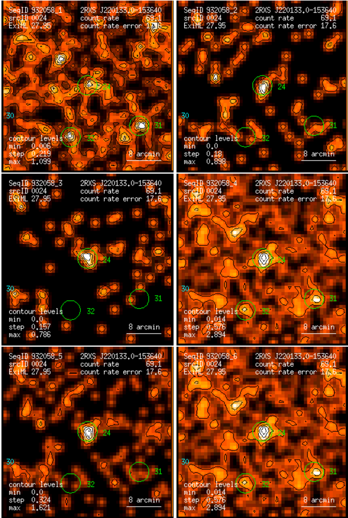
Figure 24: RASS 932058: detection 0024: band rate images, Gaussian filter: (1) PSPC channels 11 – 41, (2) 52 – 90, (3) 91 – 201, (4) 11 – 235, (5) 52 – 201, (6) 11 – 201. Broad band rates in counts/ks. Band rate contour levels in counts/ks/arcmin 2 .
