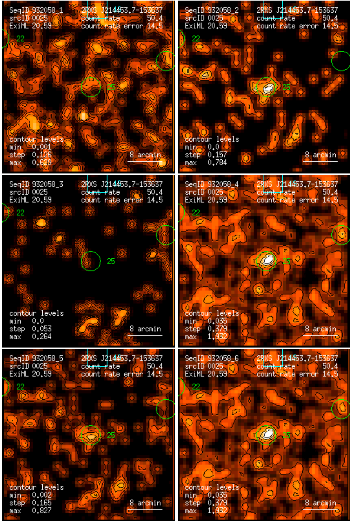
Figure 25: RASS 932058: detection 0025: band rate images, Gaussian filter: (1) PSPC channels 11 – 41, (2) 52 – 90, (3) 91 – 201, (4) 11 – 235, (5) 52 – 201, (6) 11 – 201. Broad band rates in counts/ks. Band rate contour levels in counts/ks/arcmin 2 .
