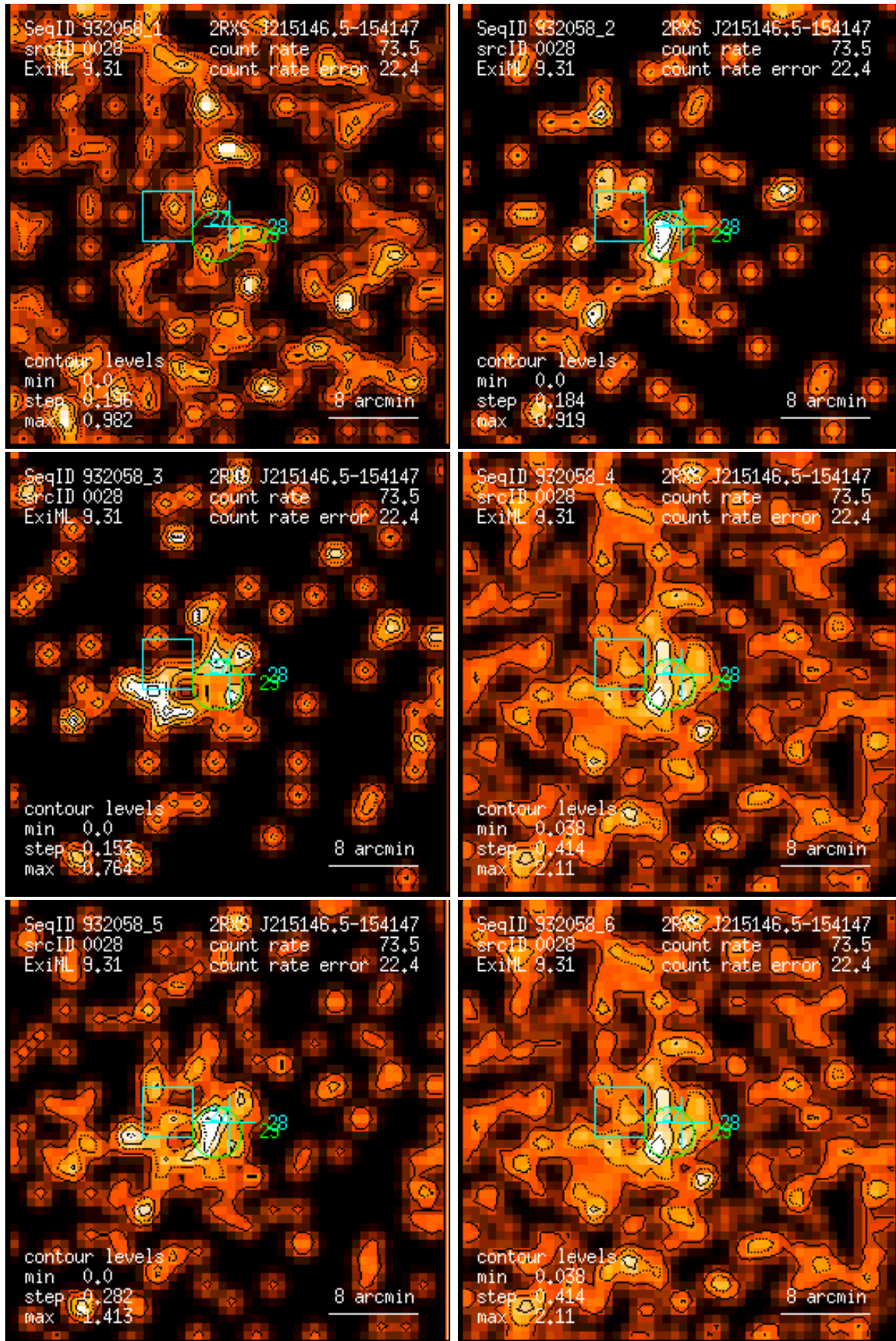
Figure 28: RASS 932058: detection 0028: band rate images, Gaussian filter: (1) PSPC channels 11 – 41, (2) 52 – 90, (3) 91 – 201, (4) 11 – 235, (5) 52 – 201, (6) 11 – 201. Broad band rates in counts/ks. Band rate contour levels in counts/ks/arcmin 2 .
