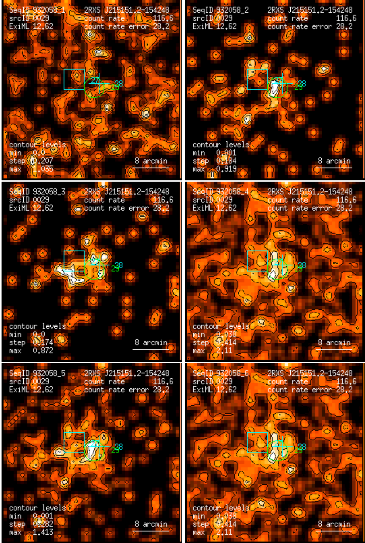
Figure 29: RASS 932058: detection 0029: band rate images, Gaussian filter: (1) PSPC channels 11 – 41, (2) 52 – 90, (3) 91 – 201, (4) 11 – 235, (5) 52 – 201, (6) 11 – 201. Broad band rates in counts/ks. Band rate contour levels in counts/ks/arcmin 2 .
